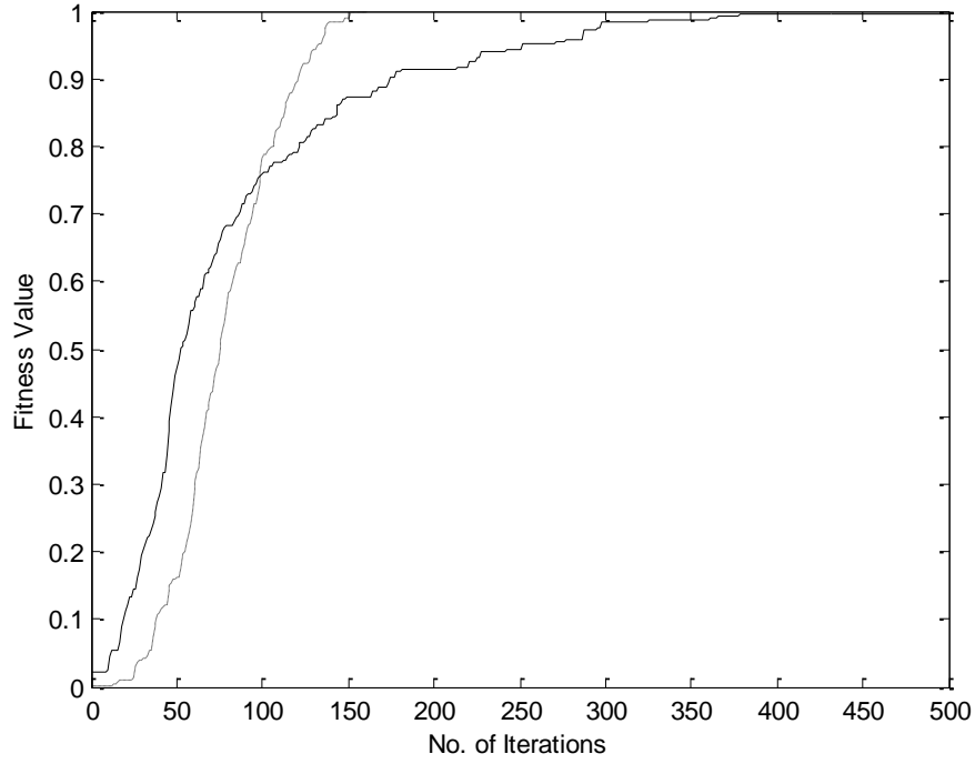
(e). The averaged fitness value of the test function f_5(\mathbf{x}) obtained by the improved (solid line) and standard (dotted line) GAs.
