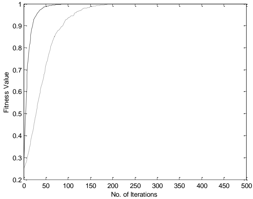
(a). The averaged fitness value of the test function f_1(\mathbf{x}) obtained by the improved (solid line) and standard (dotted line) GAs.
