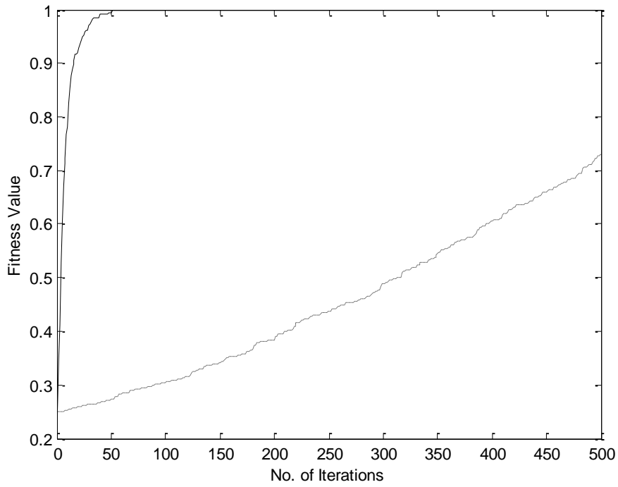
(f). The averaged fitness value of the test function f_6(\mathbf{x}) obtained by the improved (solid line) and standard (dotted line) GAs.
