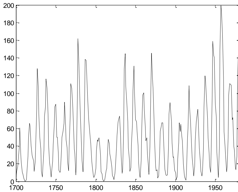
Fig. 5. Sunspot numbers from year 1700 to 1980.
