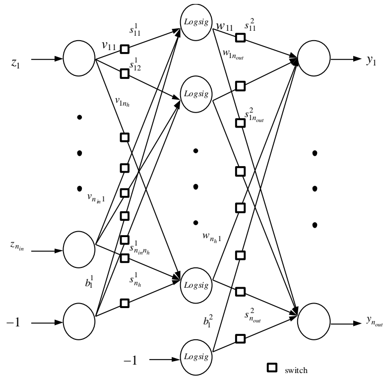
Fig. 4. Proposed 3-layer neural network.
