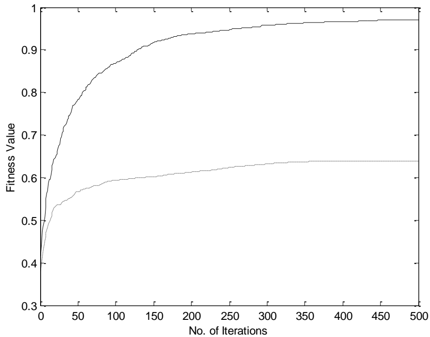
(b). The averaged fitness value of the test function f_2(\mathbf{x}) obtained by the improved (solid line) and standard (dotted line) GAs.
