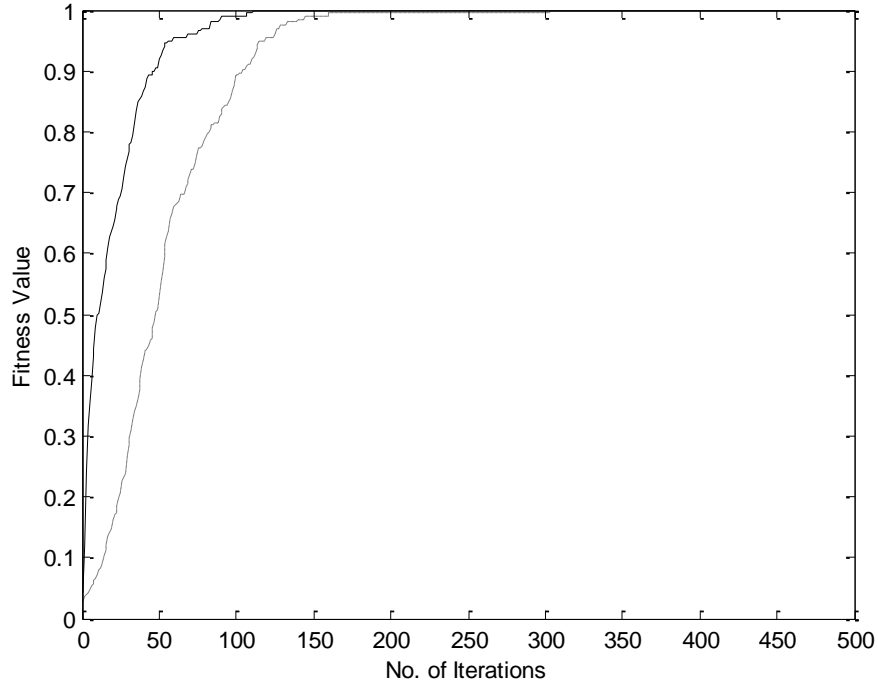
(c). The averaged fitness value of the test function f_3(\mathbf{x}) obtained by the improved (solid line) and standard (dotted line) GAs.
