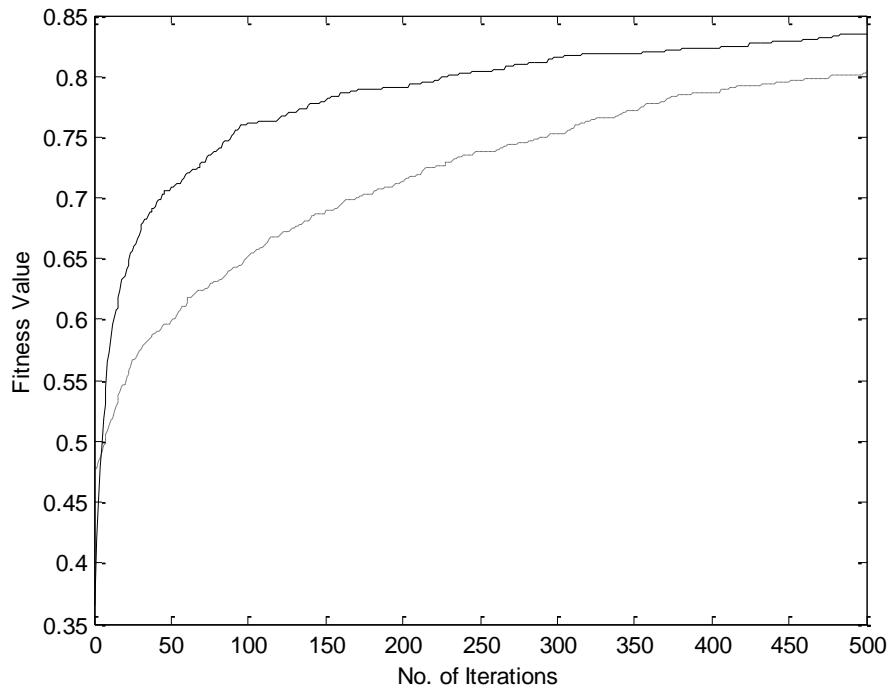
(d). The averaged fitness value of the test function f_4(\mathbf{x}) obtained by the improved (solid line) and standard (dotted line) GAs.
