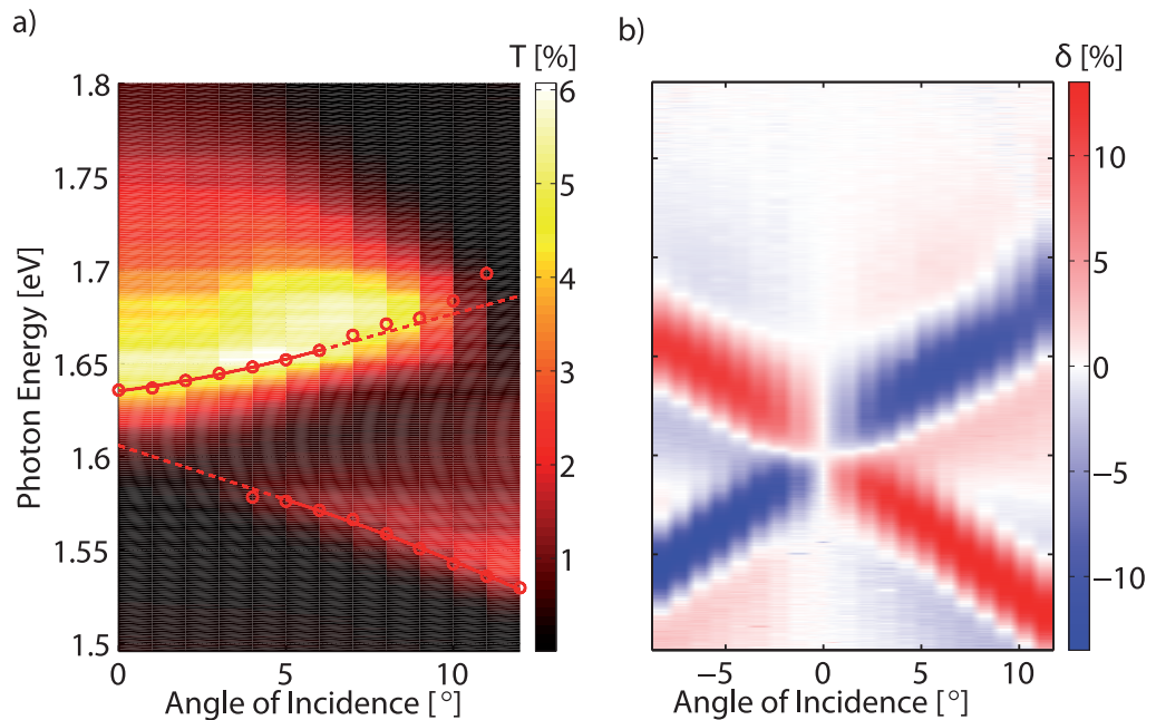
Figure 2. (a) Measured angle dependence of the transmitted light spectrum of sample 1 between \theta = 0^\circ and 12^\circ in steps of 1^\circ without applied magnetic field. Open circles show the position of the Fano resonances. The dashed lines are meant as guide to the eyes. (b) Measured angle dependence of the TMOKE in transmission on sample 1 with an applied external magnetic field of B = 80 mT. For symmetry reasons the effect vanishes for normal incidence and reverses sign when the incidence angle is reversed. For angles \theta \geq 4^\circ a remarkably high value of \delta = 13\% is reached.
