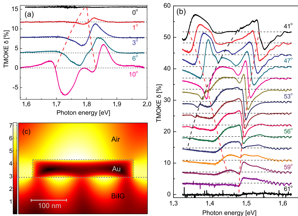
Figure 5. The TMOKE measured in transmission with sample 2 at incidence angles (a) close to k = 0 (from 0^\circ to 10^\circ ) and (b) from 41^\circ to 61^\circ , i.e. close to the edge of the first Brillouin zone. The dashed lines are guides to the eye representing the shift of the TMOKE features. Surprisingly, close to the intersection of the SPP dispersions, the curves show features whose shift can be attributed not only to the Au/BiIG magneto-plasmon (red dashed lines) but also to the Au/air SPP (black dashed line, compare figures 4(a) and (b)). At both k = 0 as well as at the 1.BZ edge, the TMOKE amplitude is zero due to symmetry considerations. The contour plot in (c) shows the calculated near field spatial distributions of the square of the absolute value of the magnetic field |H|^2 at \theta = 49^\circ and photon energy 1.38 eV.
