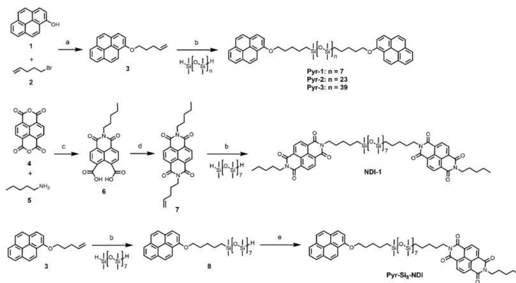
Scheme 1 Synthesis of pyrene and NDI blocks and the corresponding Pyr-1 , Pyr-2 , Pyr-3 , NDI-1 and Pyr-Si 8 -NDI . Reaction conditions: (a) K 2 CO 3 , KI, DMF, 80 °C, 24 h (89%); (b) Karstedt's catalyst, DCM, 1–2 h (51–83%); (c) DMF, microwave (i) 75 °C, 5 min, (ii) 140 °C, 15 min (22%); (d) 4-pentene-1-amine, DMF, microwave (i) 75 °C, 5 min, (ii) 140 °C, 15 min (48%); (e) NDI 7 , Karstedt's catalyst, DCM, 4 h (45%).
