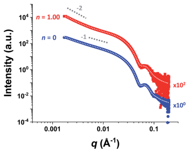
Fig. 4 Small-angle X-ray scattering (SAXS) patterns recorded for 1.0% w/w dispersions of purely HOOC-PSMA 11 -PBzMA 65 worms ( n = 1.00 , red squares) and purely H 3 COOC-PSMA 11 -PBzMA 65 worms ( n = 0 , blue circles) in n -dodecane. Indicative gradients of -1 and -2 are shown as a guide to the eye. Data fits using an established worm-like micelle model 78 are shown as dotted white lines within the experimental data. A pronounced upturn at low q is observed for the upper pattern, indicating significantly stronger inter-worm interactions in this case. This is consistent with the postulated hydrogen-bonding interactions between neighboring worms (see Scheme 3). (N.B. the n = 1.00 pattern is offset by a factor of 10^2 relative to the n = 0 pattern for the sake of clarity).
