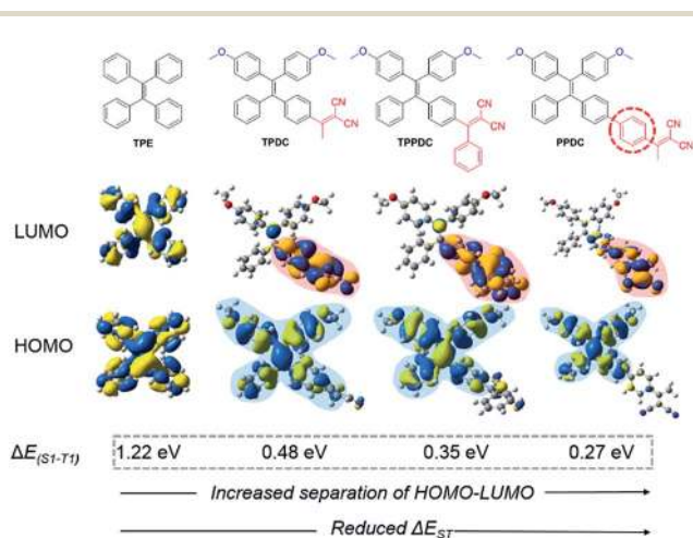
Fig. 1 Chemical structures and HOMO–LUMO distributions of TPE , TPDC , TPPDC and PPDC , optimized structures of the HOMO and LUMO at S_1 were calculated by TD-DFT (Gaussian 09/B3LYP/6-31G(d)).
