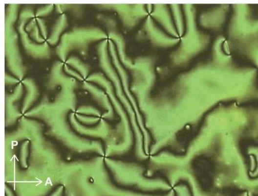
Fig. 12 Polarized optical microscopic image of cyclophane 1 at 200 °C.
