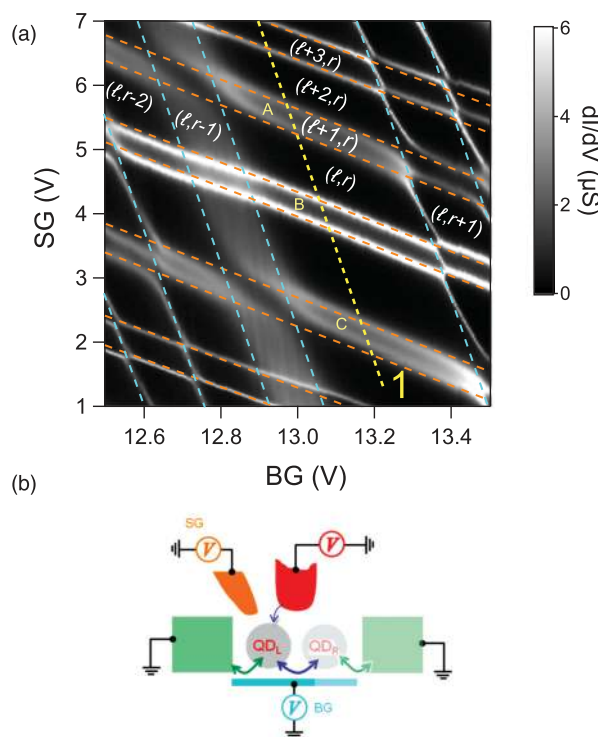
FIG. 2. (Color online) (a) Density plot of the CNT DOS measured, in the normal state ( B \sim 0.05\ \text{T} ), at zero probe voltage as a function of SG (vertical axis) and BG (bottom axis). Superimposed dotted thin lines are guides to the eyes showing the electronic levels of two isolated QDs. Orange (cyan) lines correspond to resonances of the left (right) QD. Between these dotted lines, each diamond is indexed by a pair of integer numbers, which denote the equilibrium charge on left and right dot. Here the labeling is such that \ell and r are even numbers. Avoided crossings reveal the interdot coupling. (b) Schematic of the experiment testing the DOS of a single QD ( \text{QD}_L ): by following a trajectory in the (SG, BG) plane that keeps \text{QD}_R in a “Coulomb blocked” even state [dashed yellow line 1 in (a)], the tunnel current is forced to solely go through \text{QD}_L giving access to its DOS. Dashed yellow line 1 indicates the trajectory followed to explore the DOS of a single QD in the normal and in the superconducting state shown in Figs. 3(a) and 3(b) respectively. A, B, and C correspond to the odd valleys analyzed.
