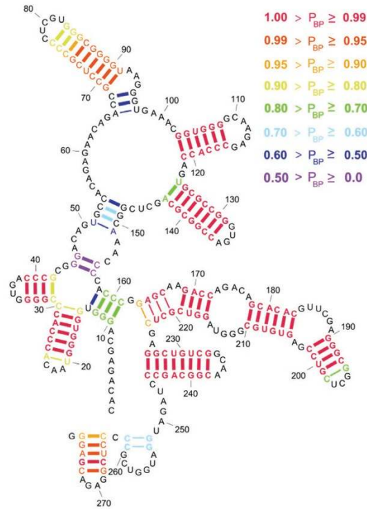
Figure 11 TurboFold structure predictions for ESH17b-7 , Synechococcus PCC6717 , and Nocardiodes NSP41 . Structures for ESH17b-7 , Synechococcus PCC6717 , and Nocardiodes NSP41 as predicted by TurboFold. The heavy lines between nucleotides represent the correctly predicted base pairs and thin lines between nucleotides represents incorrectly predicted base pairs. The colors of thick lines indicate the probability of base pairing for the nucleotides as computed by TurboFold.
