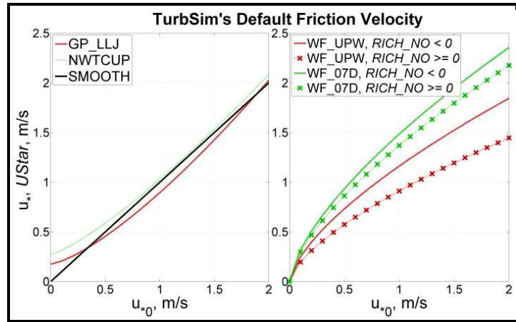
Figure 12. Default UStar as a function of diabatic friction velocity, u_{*0} (left: SMOOTH, GP_LLJ, and NWTCCUP models, right: wind farm models)
