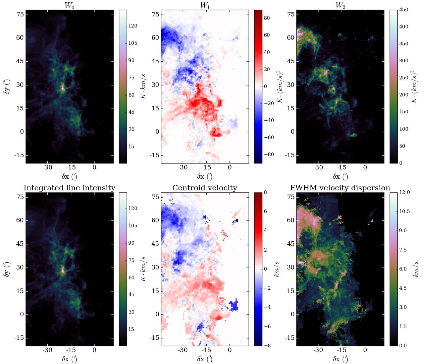
Fig. 4. Top: maps of the ^{13}\text{CO}(J=1-0) field moments in the cloud’s frame of reference. Bottom: maps of the physical quantities directly derived from each field, with the centroid velocity being simply W_1/W_0 , and the Full Width at Half Maximum (FWHM) velocity dispersion given by 2\sqrt{2\ln(2)}\sqrt{W_2/W_0} – the normalization of the FWHM corresponds to that of a field with purely Gaussian line profiles.
