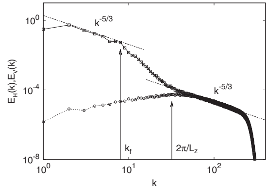
FIG. 3. Kinetic energy spectrum of horizontal (squares) and vertical (circles) velocities. Dashed lines represents Kolmogorov scaling. Parameters of the simulation: L_x = 2\pi , \ell_f/L_x = 1/8 , L_z/L_x = 1/32 , \nu_8 = 10^{-37} .
