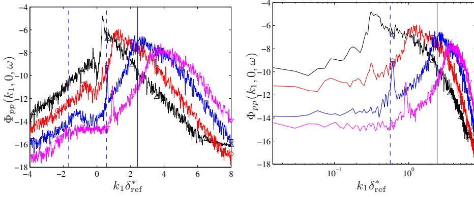
FIGURE 21. Wavenumber frequency spectra in dB (ref 1 \text{ Pa}^2 \text{ m/Hz} ) for different fixed nondimensional frequency \omega\delta^*/U_\infty : 0.25 ( \blacktriangle ), 0.85 ( \color{red}\circ ), 1.69 ( \color{blue}\square ), 2.54 ( \color{magenta}\nabla ). At the frequency \omega\delta^*/U_\infty=0.85 , the solid vertical line indicates the convective wavenumber k_c = \omega/U_c , and the dashed vertical line indicates the convected acoustic wavenumber.
