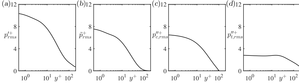
FIGURE 19. Decomposition of wall pressure fluctuations for L^+ \approx 155 and We_L = 4 \times 10^{-3} . (a) total rms pressure fluctuation, p_{rms}^+ , (b) rms stagnation pressure fluctuation, \tilde{p}_{rms}^+ , (c) rms capillary pressure p_{c,rms}^{\prime\prime+} , (d) rms turbulence pressure, p_{t,rms}^{\prime\prime+} .
