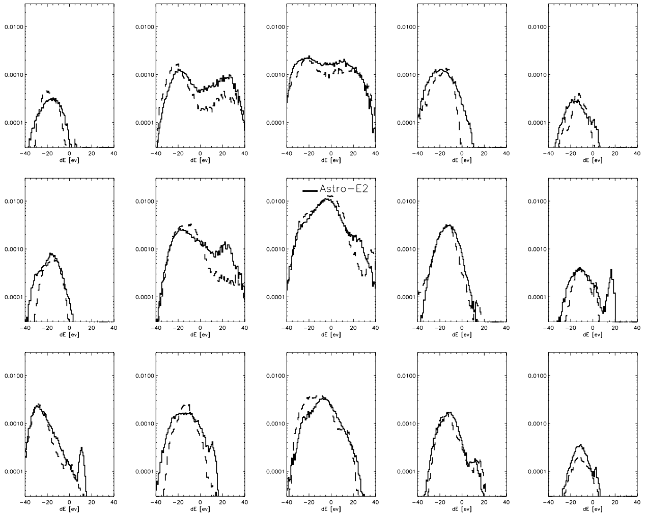
Figure 18. Distribution of the Doppler-shifted emission of the iron 6.702-keV line for 15 lines of sight through the cluster g72 . Every panel corresponds to a column of side length 300 h^{-1} kpc through the virial region of the cluster. This roughly corresponds to 1-arcmin resolution (comparable to the ASTRO-E2 specifications) at the distance of the Coma cluster. The columns from left to right correspond to -500 , -250 , 0 , 250 and 500 h^{-1} kpc impact parameter in the x -direction, and the rows correspond to -250 , 0 and 250 h^{-1} kpc impact parameter in the y -direction. The dashed lines give results for the original viscosity run, while the solid line is for the low-viscosity run. The thick bar in the centre panel marks the expected energy resolution of 12 eV as an indication for a high-resolution instrument with comparable specifications to the high-resolution X-ray Spectrometer (XRS) instrument on board ASTRO-E2 .
