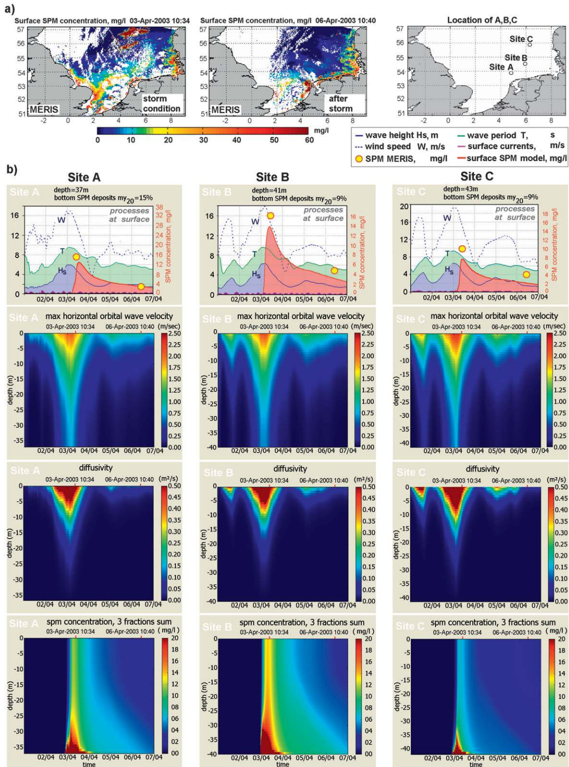
FIG. 7. The storm period 1–7 Apr 2003 in the southern North Sea. (a) MERIS scenes, presenting the SPM concentration at sea surface and locations of sites A, B, and C. The plume-shaped structure is visible during the storm but then disappears after the wave height sinks.
