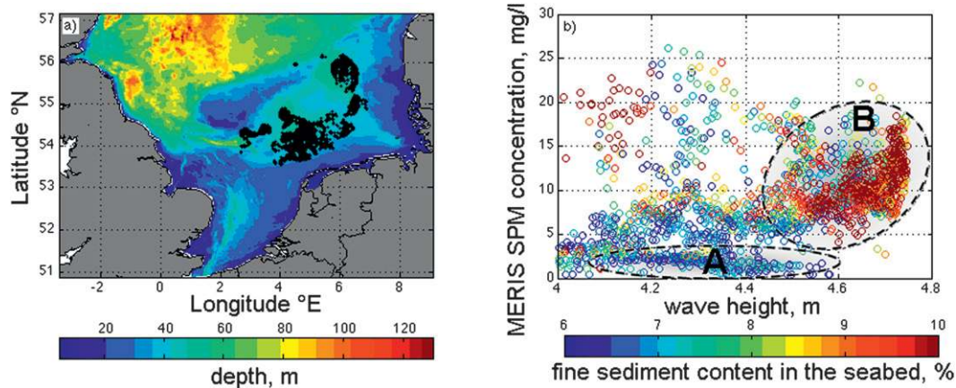
FIG. 3. (a) Selected areas ( 50 \text{ m} > \text{depth} > 30 \text{ m} ; SPM content in the seabed > 6\% ; and H_s > 4 \text{ m} , black areas) on the topography map in the North Sea and (b) scatterplot of significant wave height and MERIS SPM concentration in these areas in 2003 [colors represent percentage of SPM mass content (grain size < 20 \mu\text{m} ) in the seabed].
