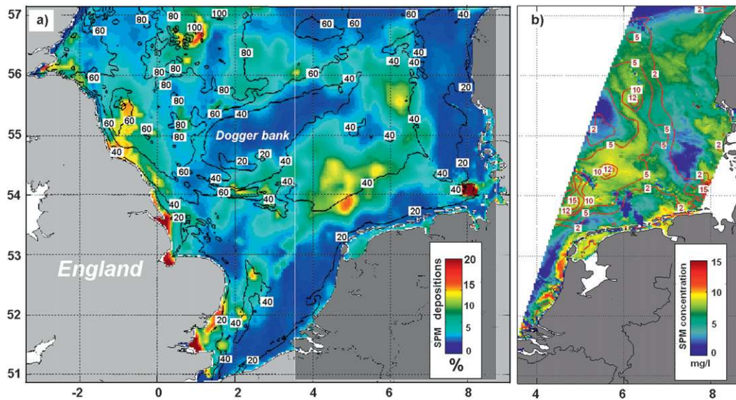
FIG. 2. (a) Seabed distribution of the fine-sediment (grain size, O < 20 \mu\text{m} ) fraction (colors in percentage of sediment mass content) and bathymetry (lines; depth in meters) in the southern North Sea and (b) the surface SPM concentration derived from MOS with the typical plume-shaped structure (the optical image seen in Fig. 1) during the storm on 4 Feb 2000 (isolines show percentage of sediment mass content).
