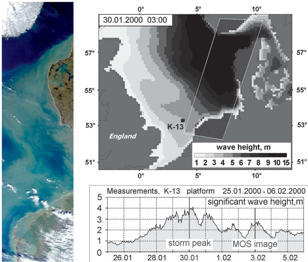
FIG. 1. Storm events in the North Sea at 29 Jan–4 Feb 2000 (the storm peak was at about 0300 UTC 30 Jan 2000). (left) Optical MOS image of German Bight on 3 Feb 2000 and (right) significant wave height in the North Sea at the storm peak.
