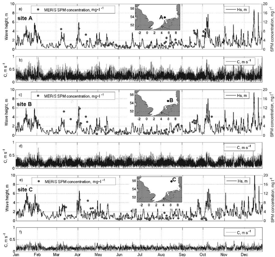
FIG. A1. Time series at A, B, and C in the North Sea in 2003 (geographical locations are shown on the map insets) of (a),(c),(e) MERIS SPM concentration (dots, right axis) and significant wave height (line, left axis). (b),(d),(f) Surface current velocity.
