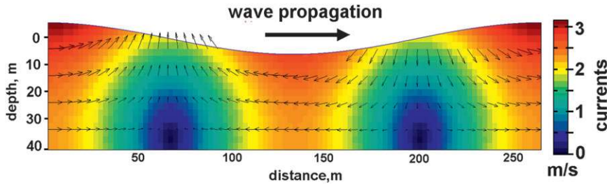
FIG. 4. Orbital wave motion. Velocity field produced by wave H_s = 10 m, T = 15 s, L = 265 m, and depth = 40 m based on the linear theory. The magnitude of velocity vector is shown by the color.
