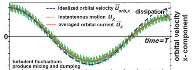
FIG. 5. Scheme of the wave damping by turbulent diffusion (no wind) for one orbital component during one wave period (horizontal axis is the time during T ). The instantaneous motion u_x (green) includes fluctuations and results the averaged orbital current \overline{u}_x (red), which differs from the idealized \overline{u_{orb,x}} (blue) because of dissipation.
