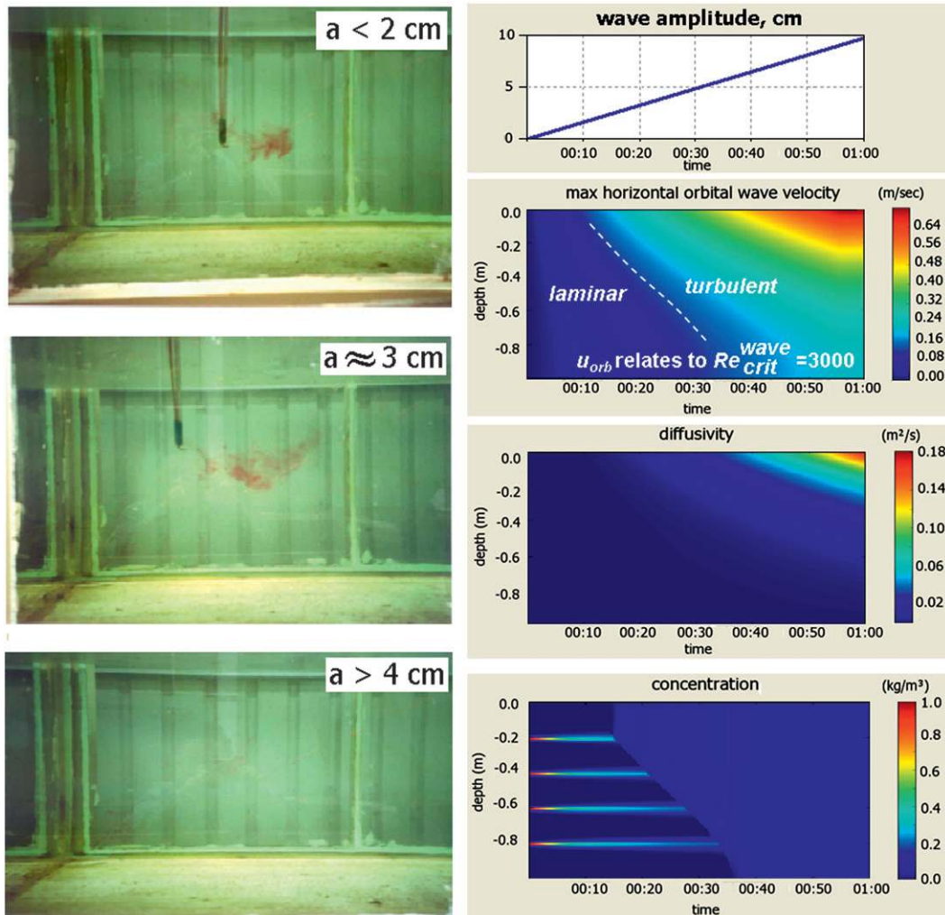
FIG. 6. Experiment in the water tank: (left) Ink is injected (no wind, no currents) for different wave amplitude and (right) reproducing of the experiment by numerical simulation.
