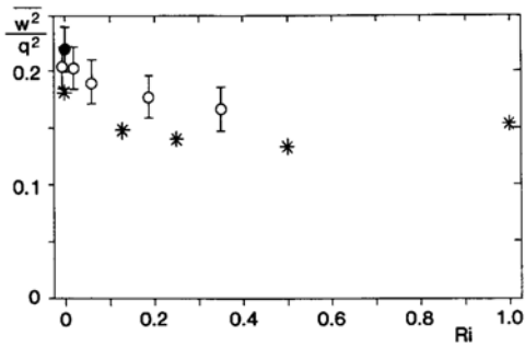
FIG. 7. Vertical velocity variance w'^2 relative to twice the kinetic energy of turbulent velocities q^2 = u'^2 + v'^2 + w'^2 versus Ri. Data from Rohr (1985) in saltwater (circles with error bars), from Tavoularis and Corrsin (1985) for air (full circle with error bar), and the LES results (stars).
