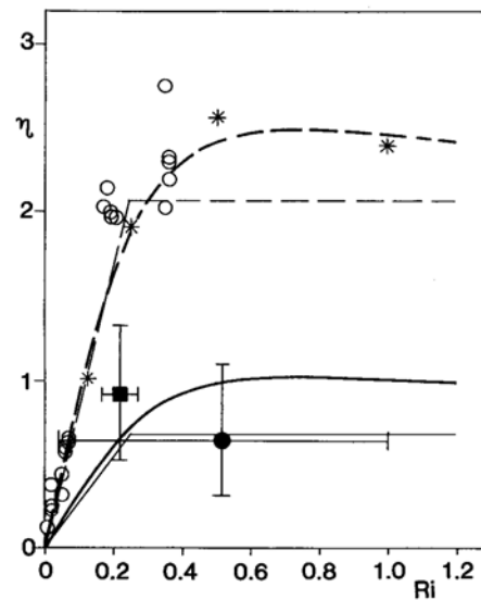
FIG. 8. Potential energy over kinetic energy of vertical motions, \eta = N^2 q^2 / \zeta_N^2 w'^2 , versus Ri. Data from Rohr (1985) in saltwater (circles), from the LES results (stars), from Nieuwstadt (1984) (full square with error bars), and from Hunt et al. (1985) (full circle with bars indicating the maximum variations of the measured data). The thick curve depicts the model, Eq. (32) for air; the dashed curve is the result for saltwater. The thin straight lines correspond to \eta = Ri_f^2 for Ri \leq 0.25 , and \eta = \zeta_N^2 for Ri > 0.25 , according to Eqs. (15) and (16), and Table 2.
