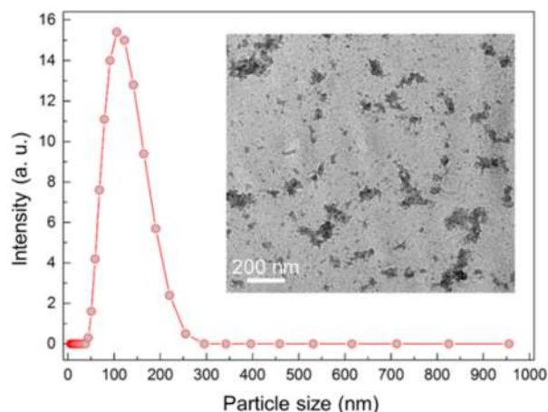
Figure 1. Particle size distribution of PDA nanoparticles. The graph shows the particle size distribution of PDA nanoparticles which were prepared after oxidization of 100 \mu\text{M} DA solution for 3 h in the presence of 20 mM NaOH. Inset shows the TEM images of the purified DA oxidization solution showing the polydisperse and irregularly shaped PDA nanoparticles.
