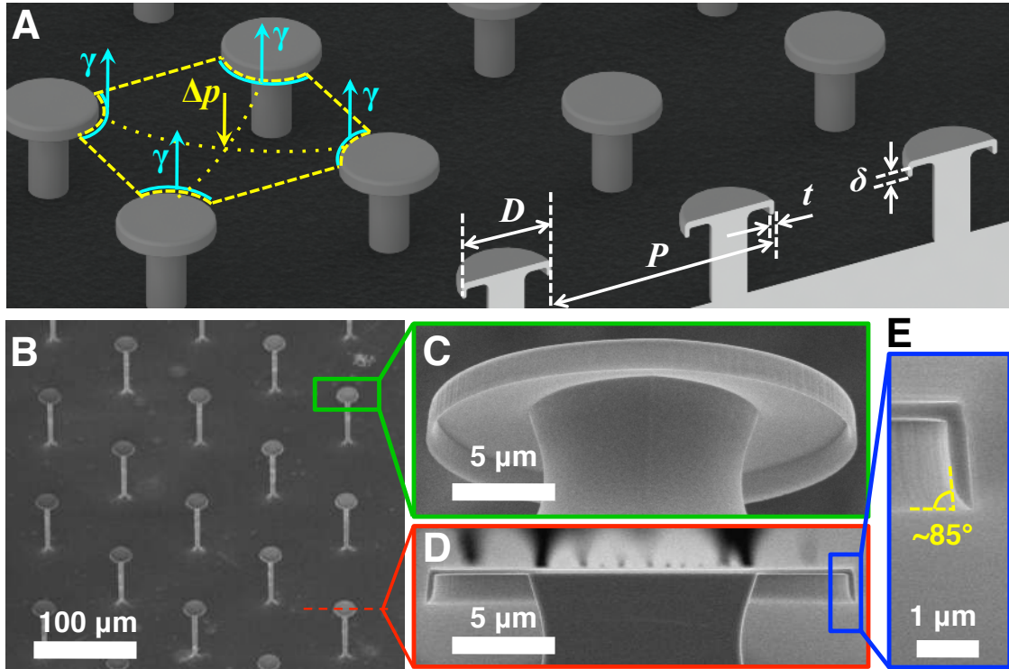
Fig. 3. Design and fabricated results of the SiO 2 surface. (A) Designed surface of micro-posts with doubly re-entrant nano-overhangs. As key geometric parameters, D is the post top diameter, P is the center-to-center distance (i.e., pitch) between adjacent posts, and \delta and t are the length and thickness of the vertical overhang. To make f_s small enough ( f_s < 6\% ), \delta and t should be shrunk to extreme values. (B to E) SEM micrographs of the fabricated surface: (B) top angled view of the square-array of circular posts with D \sim 20 \mu\text{m} , P = 100 \mu\text{m} , \delta \sim 1.5 \mu\text{m} , and t \sim 300 \text{nm} , resulting in f_s \sim 5\% ; (C) bottom angled view of one post; (D) cross-sectional view of one post, and (E) magnified cross-sectional view of the vertical overhang. Note the similarity with the ideal topology of Fig. 1C.
