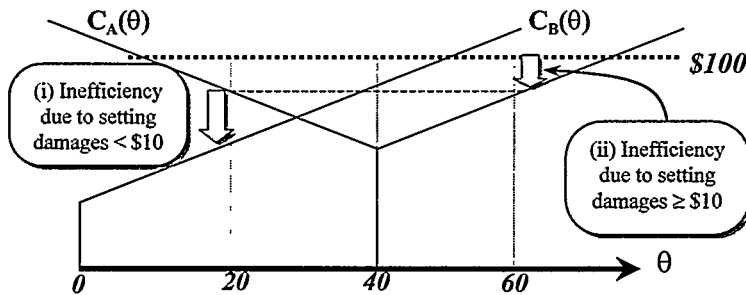
FIGURE 4. OPTIMAL CONTRACT TRADES OFF TWO TYPES OF INEFFICIENCY; \lambda = 1 , \alpha = 40
