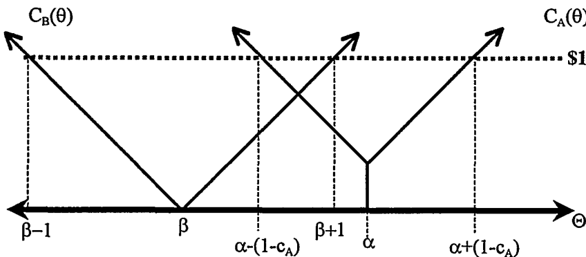
FIGURE A1: RELATIONSHIP BETWEEN PROJECT TYPE AND PLAYER SPECIALTY
