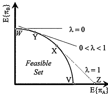
FIGURE A2: A GRAPHICAL INTERPRETATION OF A ’S WELFARE WEIGHT ( \lambda )
