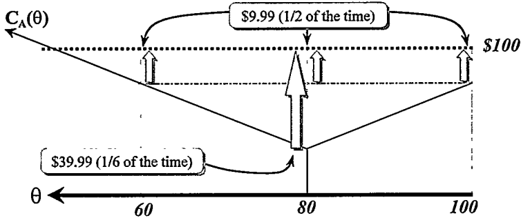
FIGURE 3. B PREFERS DAMAGES THAT OVER-DETER THE AGENT FOR “FRINGE” PROJECTS
