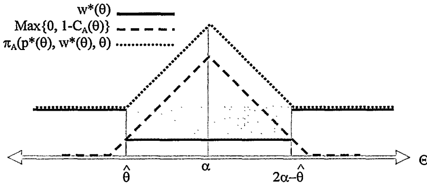
FIGURE A3: "STRIKE PRICE" FOR AUTHORIZATION IMPLICIT IN w^*(\theta) ; \lambda < 1 .
