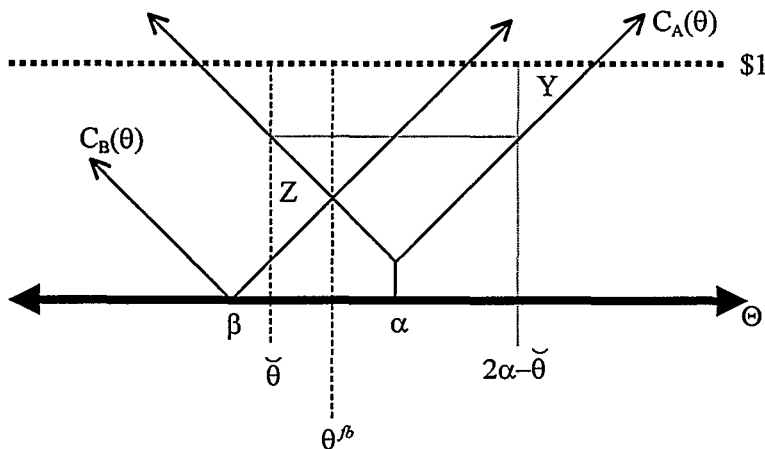
FIGURE A4: OPTIMAL CONTRACT TRADES OFF PRODUCTION INEFFICIENCIES Y AND Z .
