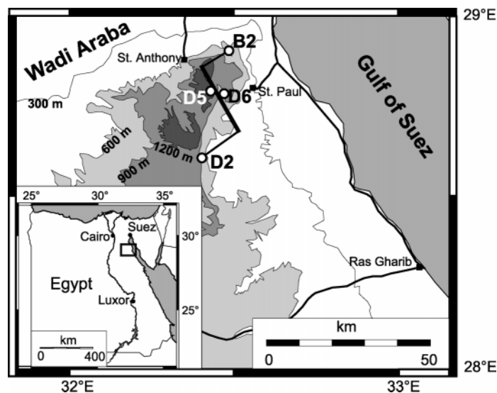
Figure 1. Location map with studied sections projected on line perpendicular to direction of platform progradation. Contours indicate elevations of Galala Mountains.
