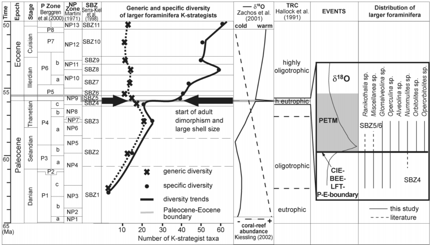
Figure 2. Biostratigraphy and comparison of trends in evolution and distribution of larger foraminifera, \delta^{18}\text{O} isotopes, coral-reef abundance, and trophic resource continuum (TRC). Inset: Events associated with the Paleocene-Eocene (P-E) boundary: CIE—carbon isotope excursion; BEE—benthic extinction event; LFT—larger-foraminifera turnover; PETM—Paleocene-Eocene thermal maximum.
