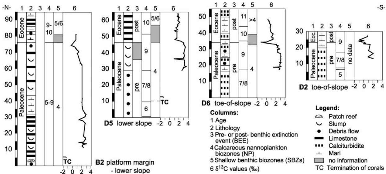
Figure 3. Biostratigraphic and chemostratigraphic correlation of studied platform-margin to toe-of-slope sections.
