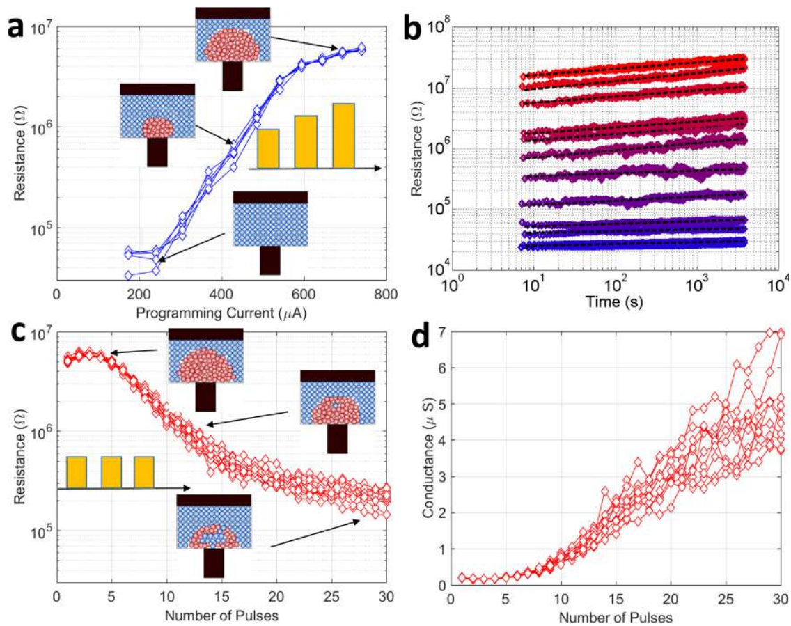
FIG. 3. (a) Characteristic programming curves that show the achievable resistance values as a function of partial RESET pulses with varying amplitude. This bi-directional curve is typically employed to achieve a desired resistance value using iterative programming. (b) Temporal fluctuations associated with the resistance values due to structural relaxation of the amorphous phase as well as 1/f noise. (c) Characteristic accumulation curves that show the evolution of resistance values as a function of the successive application of a SET pulse with the same amplitude. Due to the crystallization dynamics, there is a progressive reduction in the size of the amorphous region and the resulting device resistance. (d) Illustration of the accumulative behavior where the progressive increase in device conductance is depicted in a linear scale.
