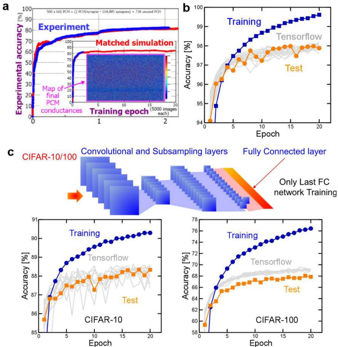
FIG. 10. (a) A mixed hardware/software demonstration of the concept of training deep neural networks using PCM devices. The training and test accuracies as a function of the number of training epochs are shown. 24 (b) and (c) The classification accuracy is shown to increase the accuracy of the mixed-hardware-software experiment to software-equivalent levels with the use of a “3T1C” circuit structure in conjunction with the PCM devices, 25 both for (b) MNIST handwritten digits and for (c) transfer learning experiments involving CIFAR-10 and CIFAR-100 datasets.
