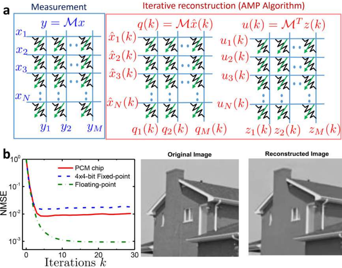
FIG. 6. (a) Compressed sensing involves one matrix-vector multiplication. Data recovery is performed via an iterative scheme, using several matrix-vector multiplications on the very same measurement matrix and its transpose. (b) An experimental illustration of compressed sensing recovery in the context of image compression is presented, showing 50% compression of a 128 \times 128 pixel image. Adapted from Ref. 21. The normalized mean square error (NMSE) associated with the reconstructed signal is plotted against the number of iterations.
