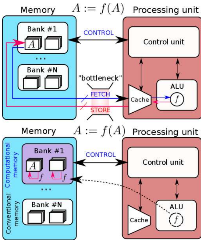
FIG. 4. “In-memory computing,” computation is performed in place by exploiting the physical attributes of memory devices organized as a “computational memory” unit. For example, if data A is stored in a computational memory unit and if we would like to perform f(A) , then it is not required to bring A to the processing unit. This saves energy and time that would have to be spent in the case of conventional computing system and memory unit. Adapted from Ref. 19.
