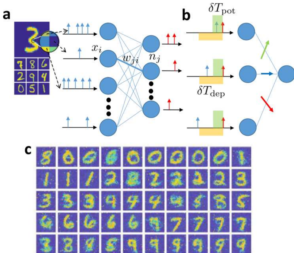
FIG. 16. (a) A spiking neural network architecture for unsupervised learning of handwritten digits. (b) Schematic illustration of the modified STDP rule. (c) The synaptic weight map corresponding to the 50 output neurons as stored in the PCM-based synapses through the unsupervised learning scheme. 45
