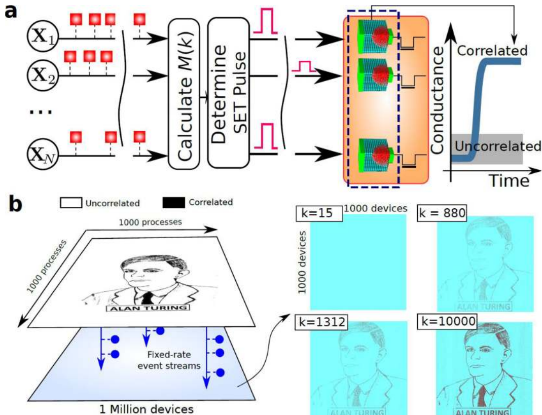
FIG. 7. (a) By interfacing binary random processes to PCM devices, it is possible to learn the temporal correlations between the processes in an unsupervised manner. (b) Experimental demonstration of the concept using a million PCM devices. 19 The result of the computation is imprinted as conductance values in the memory array.
