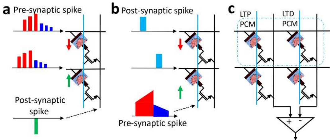
FIG. 14. (a) Two synaptic elements, each comprising a PCM device and a transistor. The transistor just serves as a switch in this configuration. To implement STDP, the pre-synaptic neuronal spike initiates a sequence of pulses with varying amplitude and the post-synaptic neuronal spike initiates a single pulse with opposite polarity. (b) Two synaptic elements, each comprising a PCM device and a transistor. In this configuration, the transistor plays an active role in the realization of synaptic plasticity. The pre-synaptic neuronal spike initiates a voltage pulse applied to the gate of the transistor and the post-synaptic neuronal spike initiates a pulse applied to the top electrode of the PCM device. (c) A synaptic element comprising two PCM devices organized in a differential configuration.
