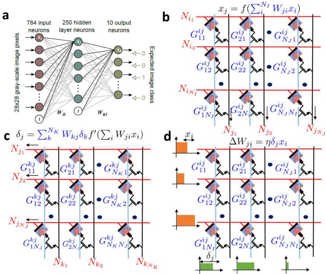
FIG. 9. (a) A prototypical two-layer neural network to classify handwritten digits based on the MNIST dataset. (b) The matrix-vector multiplications associated with the forward pass can be implemented with O(1) complexity. (c) The backward pass involves a multiplication with the transpose of the matrix representing the synaptic weights, which can be realized with O(1) complexity. (d) The synaptic weight update can also be achieved in place in O(1) time complexity.
