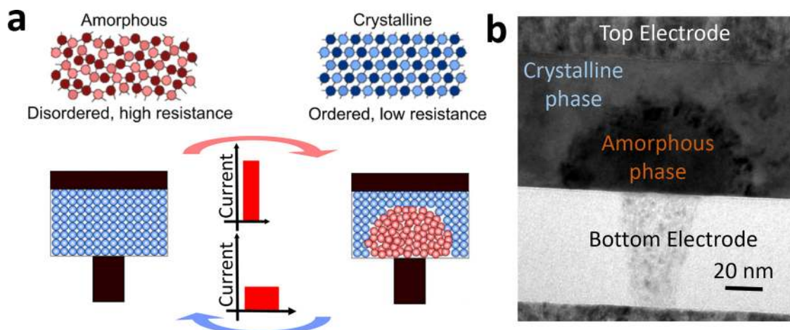
FIG. 2. (a) Phase-change memory is based on the rapid and reversible phase transition of certain types of materials between crystalline and amorphous phases by the application of suitable electrical pulses. (b) Transmission electron micrograph of a mushroom-type PCM device in a RESET state. It can be seen that the bottom electrode is blocked by the amorphous phase.
