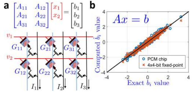
FIG. 5. (a) Matrix-vector multiplication can be performed with O(1) complexity by organizing PCM devices in a cross-bar configuration. (b) Experimental demonstration of the concept using PCM devices fabricated in the 90 nm technology node.
