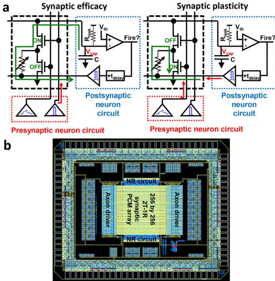
FIG. 15. (a) Synaptic efficacy and plasticity can be realized very efficiently using a synaptic element comprising 1 PCM device and two transistors. (b) A neuromorphic core comprising 64 000 such synaptic elements. 41
