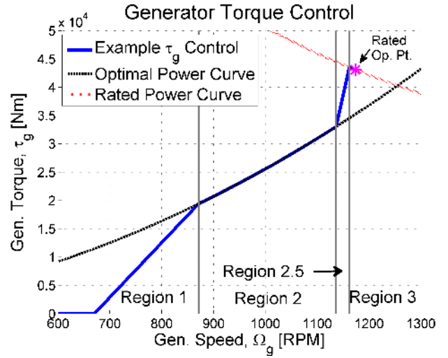
Fig. 4. An example of the generator torque control in different operating regions, as described in [8].
