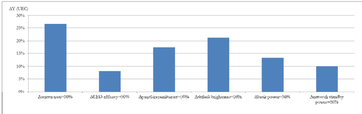
Figure C-1. UEC Sensitivity to Technical Factors (32" LED-LCD TV, P_{\text{network standby}}=4 \text{ W} )
