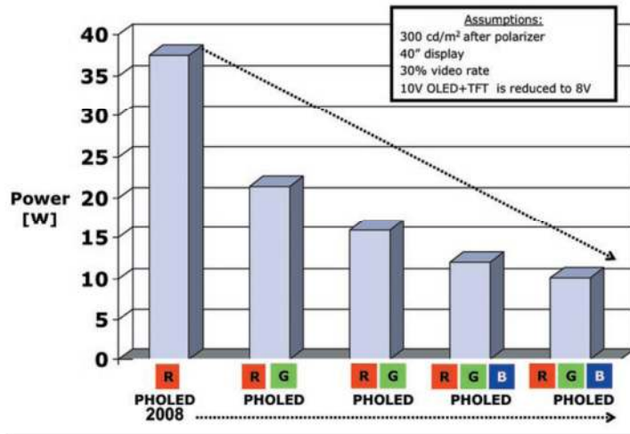
Figure 4-23. Power Consumption Roadmap for 40-inch (101.6-cm) OLED TV Panels
