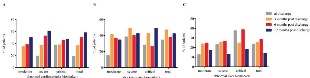
Figure 2. Frequencies of abnormal biomarkers (in %) of recovered patients with COVID-19 at discharge, as well as 3, 6, and 12 months follow-up visits post-discharge. Symptom frequencies are stratified by disease severities (moderate, severe, and critically ill). (A) Abnormal cardiovascular biomarkers; (B) abnormal renal biomarkers; (C) abnormal liver biomarkers. Abbreviation: COVID-19, coronavirus disease 2019.
