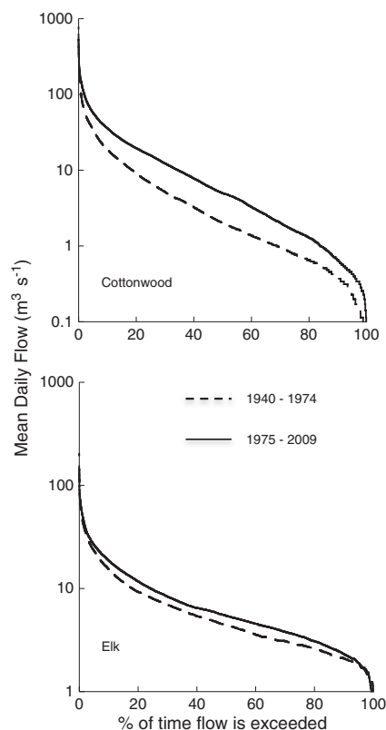
Figure 7. Representative flow duration curves for a river with channel widening (Cottonwood) and one without (Elk). High flows are toward the left and low flows toward the right. Rivers such as the Cottonwood, which had significant increases in total annual water yield, showed increases in nearly all flow regimes
