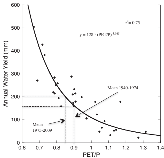
Figure 3. Calibration of the response of water yield to climate (precipitation), and cropping characteristics using annual values for the initial 35 year period (1940–1974); an example for the Blue Earth watershed. The mean PET/P ratio changed from 0.9 to 0.85 from the first period to the second (dashed lines). Applying this change in PET/P to the empirical relationship predicts a 33.5 mm increase in annual water yield in the second time period due climate and crop conversions combined
