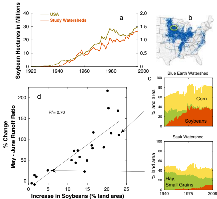
Figure 1. (a) Twentieth century increase in soybean acreage in the USA and for the combined 21 watersheds evaluated in this study. (b) Soybean growing region of the USA; yellow circle encompasses the 21 study watersheds. (c) Exemplary watersheds illustrating different levels of crop conversion among watersheds. (d) Relationship between the conversion to soybeans and the change in May–June runoff ratio. The conversion to soybeans subsumes multiple factors affecting hydrology. Change over time is expressed as the difference between the median values of the two time periods: 1940–1974 and 1975–2009
