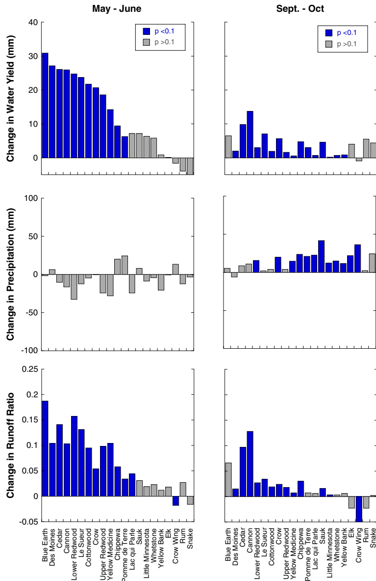
Figure 4. Seasonal changes in water yield (flow volume/watershed area), precipitation, and runoff ratio (water yield/precipitation) for 21 watersheds tributary to the Upper Mississippi River. Changes represent the difference between median values for two 35-year periods (1940–1974 and 1975–2009). Annual changes follow a similar pattern, with water yield and runoff ratios increasing by >50% in watersheds with significant trends
