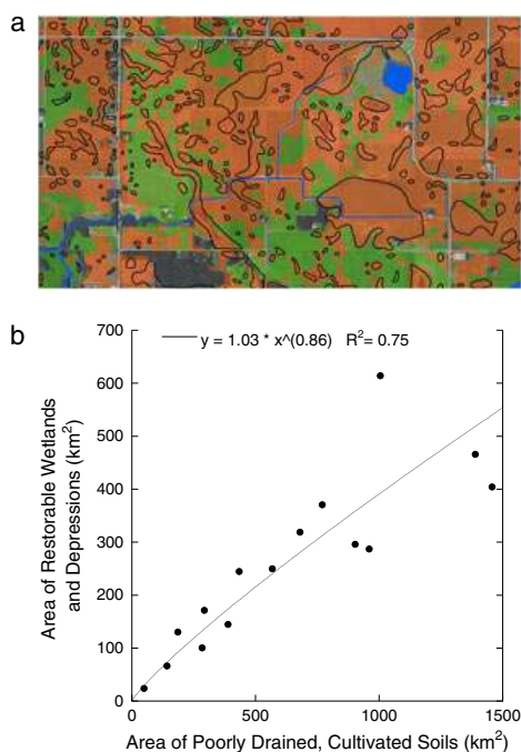
Figure 2. Predictive relationship between drained depressions and poorly drained cultivated soils for areas inventoried within the study watersheds. Upper image (a), from the Le Sueur watershed, shows cultivated soils (green), poorly drained cultivated soils (brown) drained depressions (black polygons) and existing wetlands (blue). In this example nearly all historic depressions/wetlands have been drained. Drained depression data were available for about 60% of the area in the 21 watersheds. The above regression (b) and the total amount of poorly drained cultivated soils in each watershed were used to estimate the total area of drained depressions
