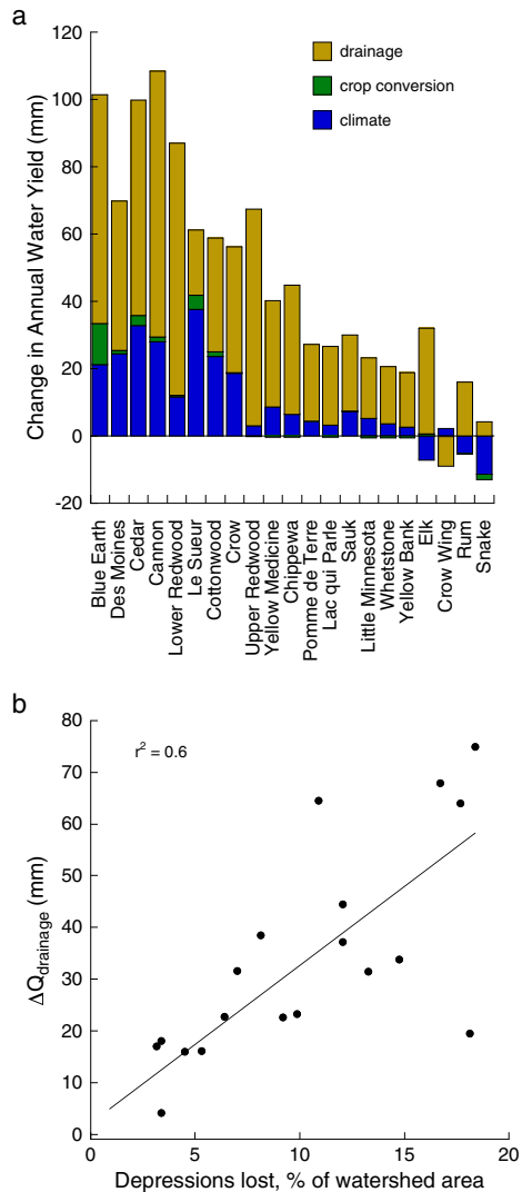
Figure 5. (a) Apportionment of changes in mean annual water yield for each watershed. In rivers with significant changes in flow, climate and crop conversions account for less than half of the total change in water yield. Excess water yield is the portion that cannot be attributed to changes in crop ET and climate and is hypothesized to result from artificial drainage ( \Delta Q_{\text{drainage}} ). (b) The increase in water yield attributed to drainage is strongly correlated with the loss of depressional areas, supporting the argument that the change in flow not accounted for by climate and crop conversion is a result of artificial drainage networks
