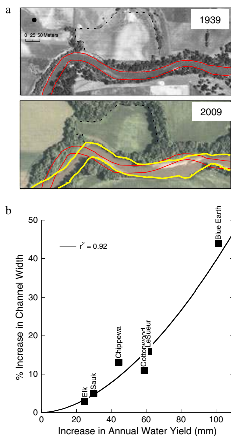
Figure 6. Channel widening related to increases in flow. (a) Photos show widening on the Blue Earth River. Red line is the bankfull width in 1939; yellow line is 2009. (b) Widening is the percent change in mean width between the two time periods (1940–1974 vs 1975–2009) and is strongly related to the increase in annual water yield. The four rivers with the greatest amount of widening are all tributaries to the Minnesota River, which has experienced a 33% (Table S2) increase in mean channel width over the same time period
