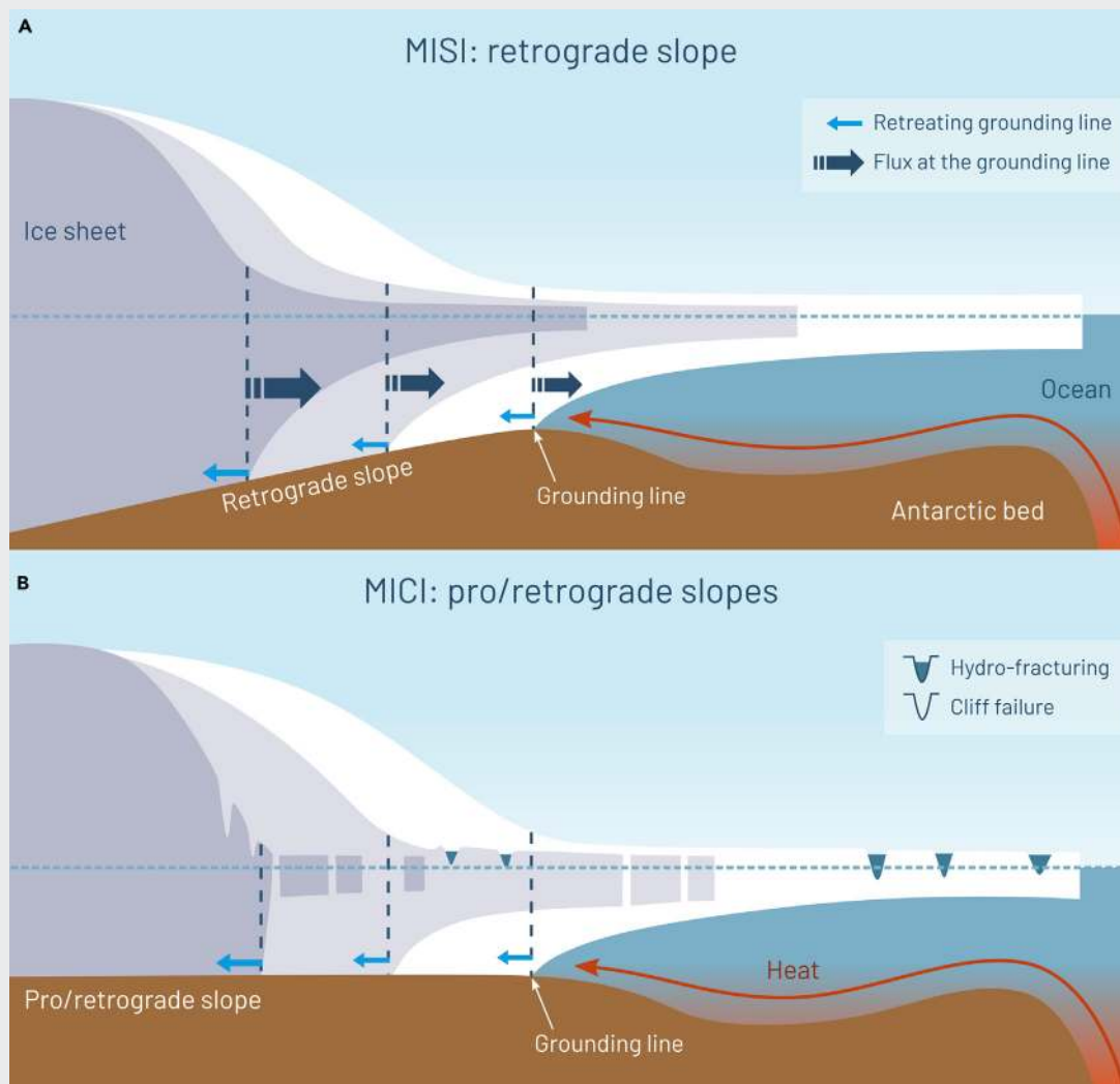
Box 1 Figure. Schematic of key processes leading to rapid ice loss at marine glacier and ice-sheet margins.
