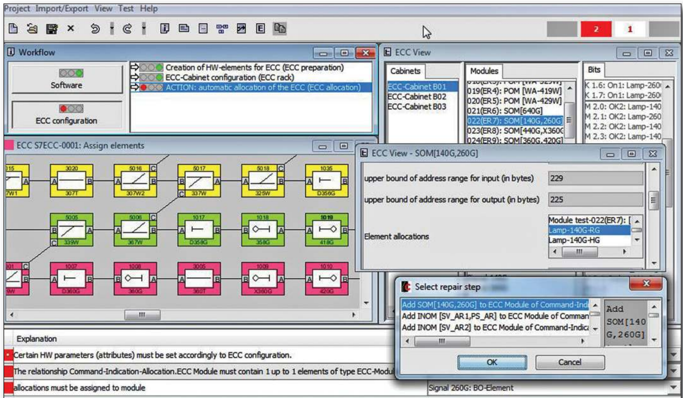
Figure 4. A Configurator for Railway Interlocking Systems.
