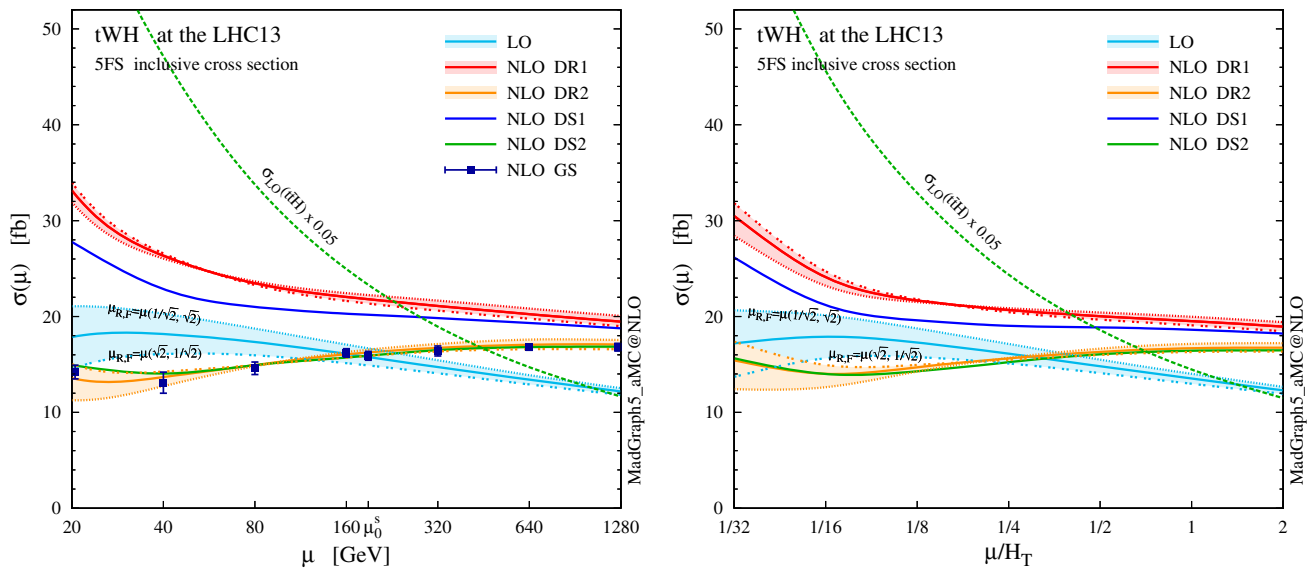
Fig. 11 Scale dependence of the total cross section for pp \rightarrow tW^-H and t\bar{W}^+H at the 13-TeV LHC, computed in the 5FS at LO and NLO accuracy, presented for \mu_F = \mu_R \equiv \mu using a static scale (left) and a dynamic scale (right). The NLO tWbH channels are treated using DR and DS; see Sect. 2 for more details. Furthermore, we show
