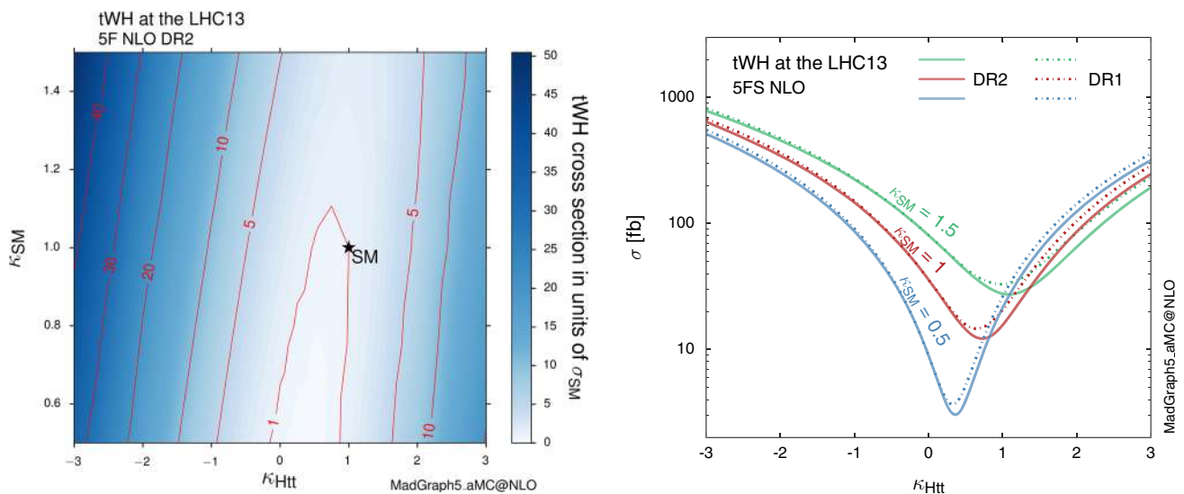
Fig. 16 Left: inclusive tWH cross sections with DR2 scanned over different values for \kappa_{\text{Htt}} and \kappa_{\text{SM}} . Note that the standard model configuration (+1, +1) almost lies in a minimum, which means the process is suited for constraining this place due to enhanced rates for deviations
