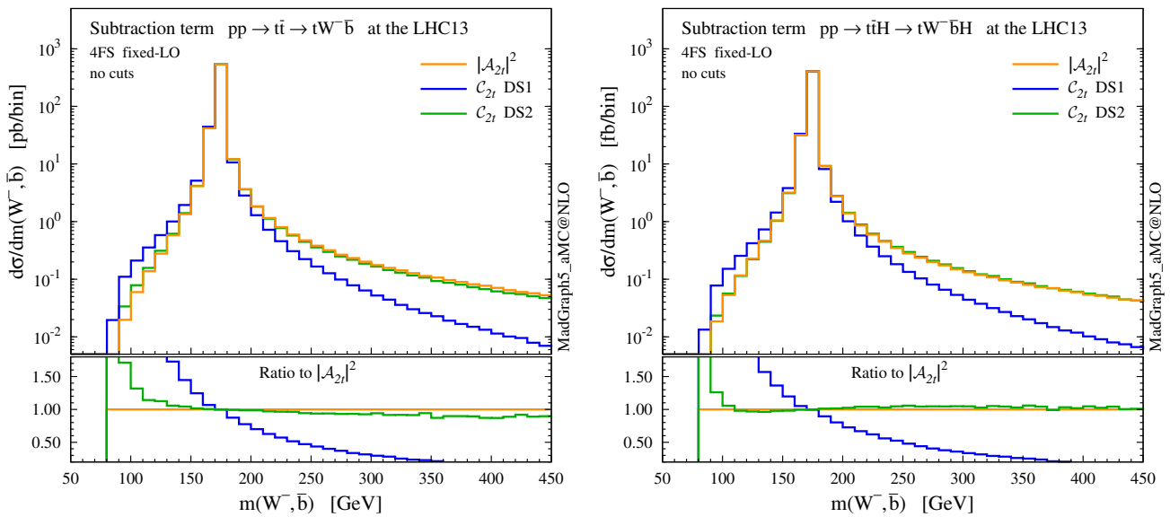
Fig. 3 Invariant mass m(W^-, \bar{b}) distributions in the pp \rightarrow tW^-\bar{b} process (left) and in the pp \rightarrow tW^-\bar{b}H process (right), for comparison between |\mathcal{A}_{2t}|^2 and C_{2t} with two different Breit–Wigner forms, DS1 and DS2
