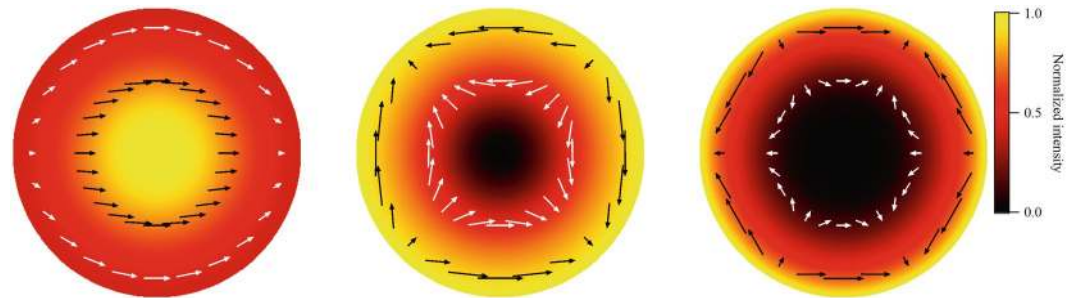
Figure 3. Electric field distribution in the upper hemisphere viewed from the z -direction (see Fig. 1), from left to right, for the fundamental ( l=1 ), second ( l=2 ) and third ( l=3 ) harmonics calculated from Eq. (5). The colour represents the field intensity. The fundamental frequency has an intensity maximum in the centre, whereas the harmonics show zero intensity at the centre. Arrows represent the direction of the electric field at a specific time.
