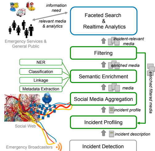
Figure 1: Twitcident architecture: (i) incident profiling and filtering of social media that is relevant to an incident (green boxes) and (ii) faceted search and realtime analytics functionality to explore and overview the media (blue box). Both types of components benefit from the semantic enrichment of the aggregated media.
