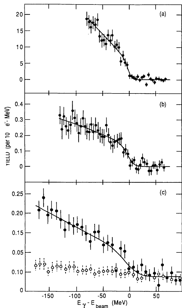
FIG. 12. Subtracted proton yields as a function of E_\gamma for the reaction {}^2\text{H}(\gamma,p)n for (a) E_\gamma \approx 0.8 GeV and \theta_{c.m.} = 90^\circ , (b) E_\gamma \approx 1.6 GeV and \theta_{c.m.} = 90^\circ , and (c) E_\gamma \approx 1.6 GeV and \theta_{c.m.} = 143^\circ . The solid lines are fits using a thick target bremsstrahlung calculation, folded with the experimental resolution, along with a nominal energy dependence of the cross section.
