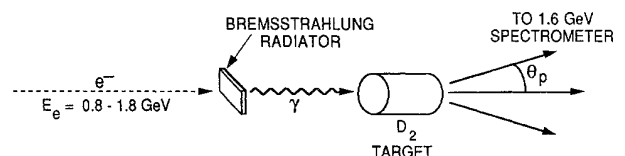
FIG. 3. Schematic of the experimental technique.
