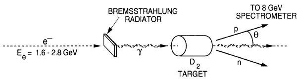
FIG. 1. The target region showing the bremsstrahlung radiator, the deuterium target, and the spectrometer pivot.
