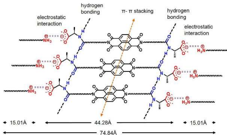
Figure 8. A tentative model for the molecular packing arrangements among the gelator molecules in the two-component co-assembled system obtained from FTIR, PXRD and SAXS data. The molecular length of dodecylamine (C12) has been used to calculate the total molecular length in the two-component co-assembled structure.
