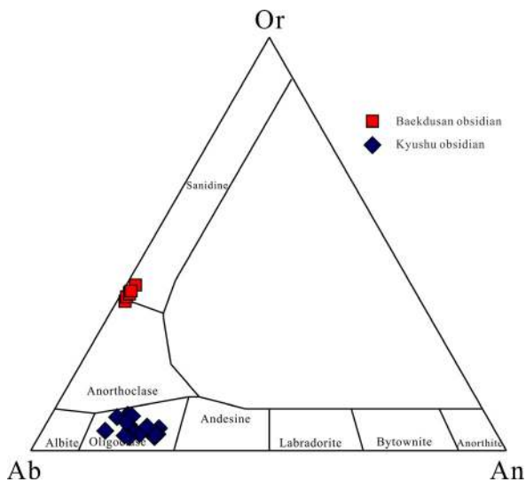
Figure 6. KAISi_3O_8(Or) - NaAlSi_3O_8(Ab) - CaAl_2Si_2O_8(An) discrimination of feldspar.
