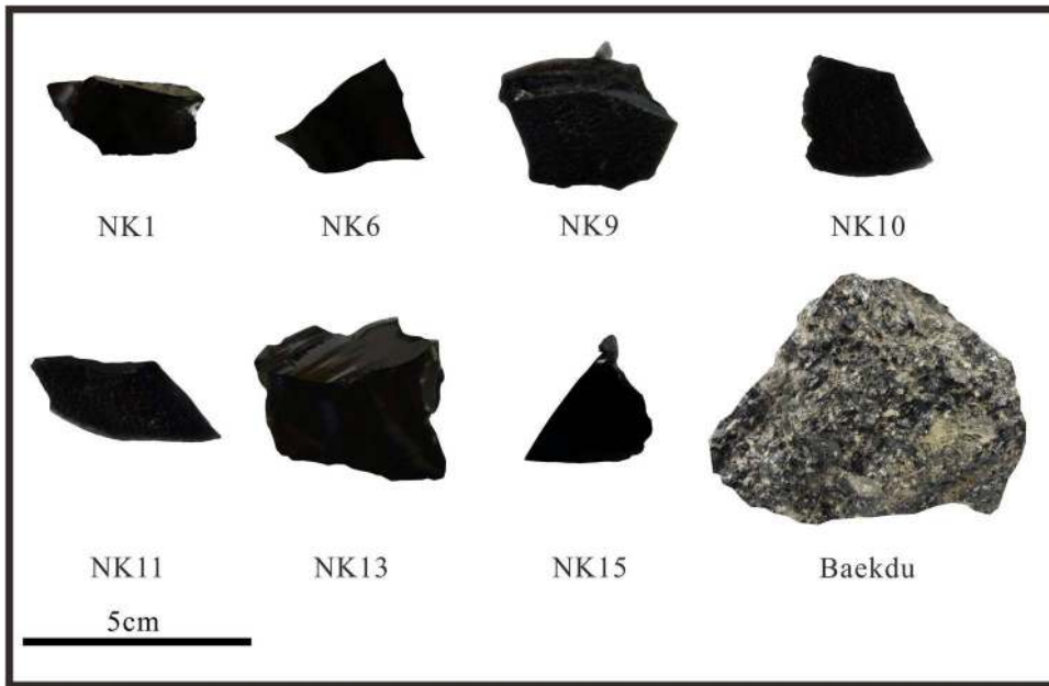
Figure 3. The Baekdusan obsidians used in this study. Seven NK obsidians were collected from a massive obsidian mine located at the southern flank of Mt. Baekdusan, and one sample, Baekdu, was from a trachytic lava layer.
