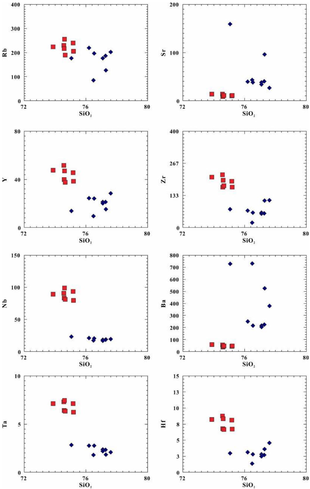
Figure 8. SiO 2 (wt.%) versus trace element contents (ppm) variation diagrams for the Baekdusan and Kyushu obsidians. The symbols are the same as Fig. 7.
