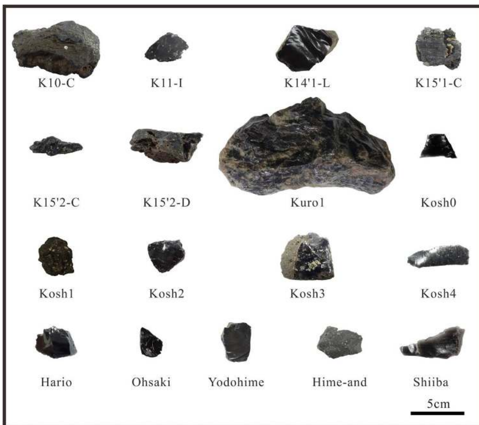
Figure 4. The Kyushu obsidians used in this study. The obsidian samples were collected from outcrops of seven localities: Koshidake (K10-C, K11-I, K14'1-L, K15'1-C, K15'2-C, K15'2-D, Kosh0, Kosh1, Kosh2, Kosh3, Kosh4), Kurogamiyama (Kuro 1), Harioshima (Hario), Ohsaki Peninsula (Ohsaki), Yodohime Higashihama (Yodohime), Himeshima (Hime-and), Shiibagawa (Shiiba).
