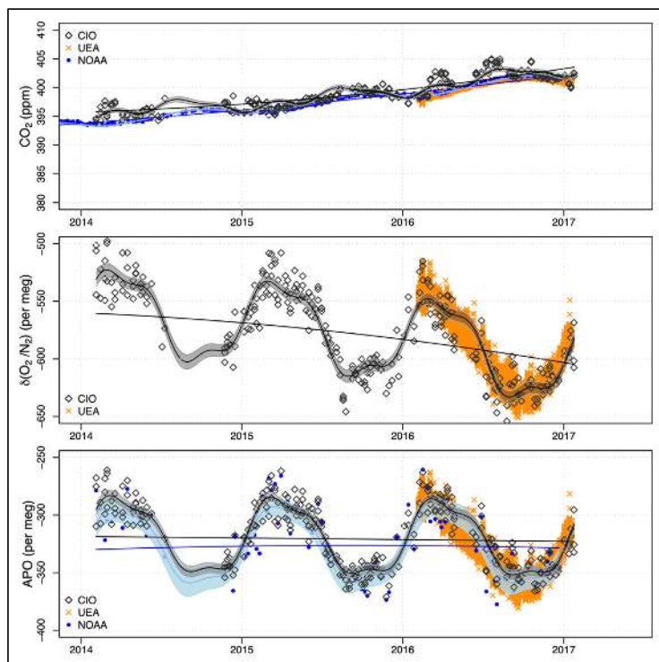
625 Figure 12: Measurements of \text{CO}_2 , \delta(\text{O}_2/\text{N}_2) , and APO at Halley conducted by CIO (black diamonds) from 2014 to 2017, and continuous measurements conducted by UEA (orange crosses) in 2016. The black lines and curves are the trends and the combined fit for measurements by CIO, respectively. The grey shaded area is the 95% CI associated with the total fit. The blue points are the in-situ continuous measurements at Halley, taken by NOAA. The blue lines and curves are the trends and the combined fits for the continuous measurements, with the lighter blue shaded area the 95% CI associated with the total fit. From the combination of all data we conclude that our \text{CO}_2 measurements must have been contaminated with inside air (human breathing).
