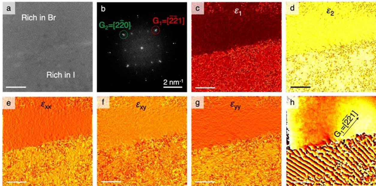
Supplementary Fig. 16 | Geometric phase analysis of the (2T)_2PbI_4-(2T)_2PbBr_4 heterostructure. a , AC-HRTEM image of the interface. b , FFT pattern. G_1 and G_2 represents two Bragg reflections. c , Maximum normal strain. d , Minimum normal strain. e , f , g , Strain mappings at different directions. \epsilon_{xx} , \epsilon_{xy} and \epsilon_{yy} represent the strain are parallel to the direction of Bragg reflections G_1 , G_1+G_2 , G_2 , respectively; These strain mappings indicate the clear interface between the substrate and epitaxy. h , Phase image with G_1=[\bar{2}\bar{2}1] . The scale bars are 40 nm. Relatively even color area shows the lattice spacing of (2T)_2PbBr_4 area are uniform and uneven color shows the lattice spacing of (2T)_2PbI_4 changes with positions regularly 5,6 . This reveals the lattice mismatch directly and implies that interfacial dislocations may exist at a certain interval to relax the lattice strain.
