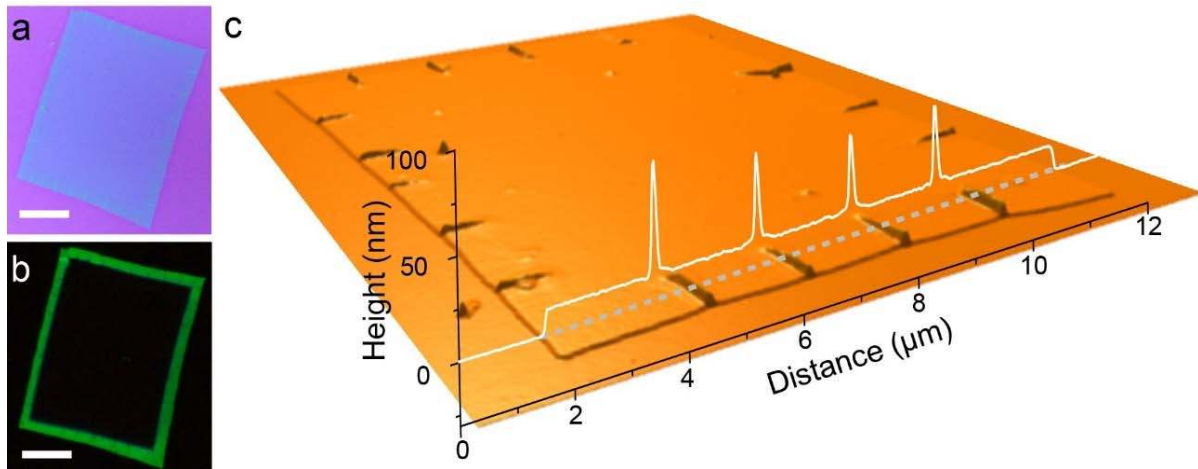
Fig. 3 | Periodic ripples in (2T)_2PbI_4-(2T)_2PbBr_4 lateral heterostructures. a, b , Optical and PL images of a one-pot (2T)_2PbI_4-(2T)_2PbBr_4 lateral heterostructure, where ripples in the (2T)_2PbI_4 region can be distinguished. The scale bars are 5\ \mu m . c , AFM image of the one-pot (2T)_2PbI_4-(2T)_2PbBr_4 lateral heterostructure with clear ripples. The height profile along the dashed line indicates the height of the ripples is around 40\sim 50\ nm .
