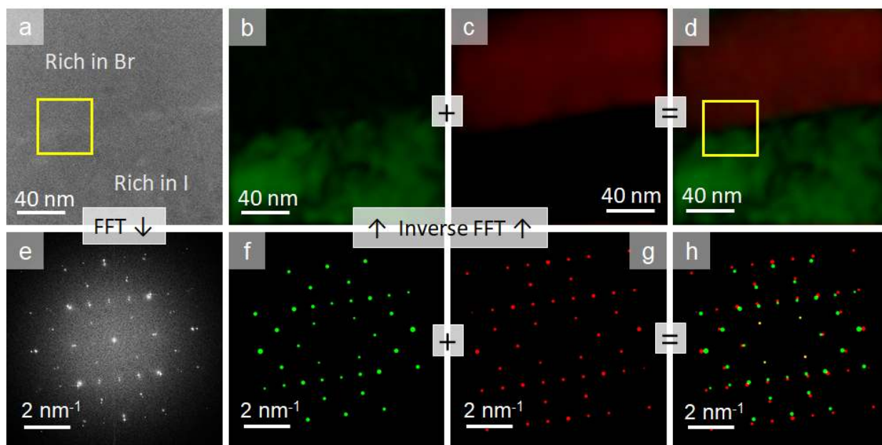
Supplementary Fig. 15 | AC-HRTEM analysis by Fourier filtering. a , AC-HRTEM image of one (2T)_2PbI_4 - (2T)_2PbBr_4 heterostructure. The yellow rectangular box denotes the Fig. 2c 1 in the main text. b , c , Inverse FFTs of (f) and (g) reveal the distinct lattice information in real space respectively. d , Superposition of (b) and (c) shows the continuous and sharp interface. False color was used for a clear view of the interface. The yellow rectangular box denotes the Fig. 2c 4 in the main text. e , FFT pattern of (a). f , g , Two masks are placed on the diffractogram (e) to filter out two different phases, respectively. h , Superposition of (f) and (g) shows the splitting diffraction spots. False color is used for differentiating two sets of spots.
