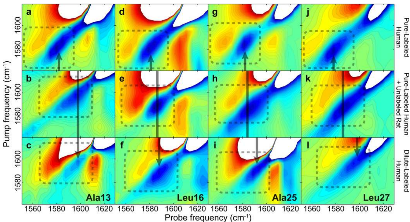
Figure 2. Rat amylin prevents human amylin from forming N-terminal, \beta -sheets at 8 hours after mixing
