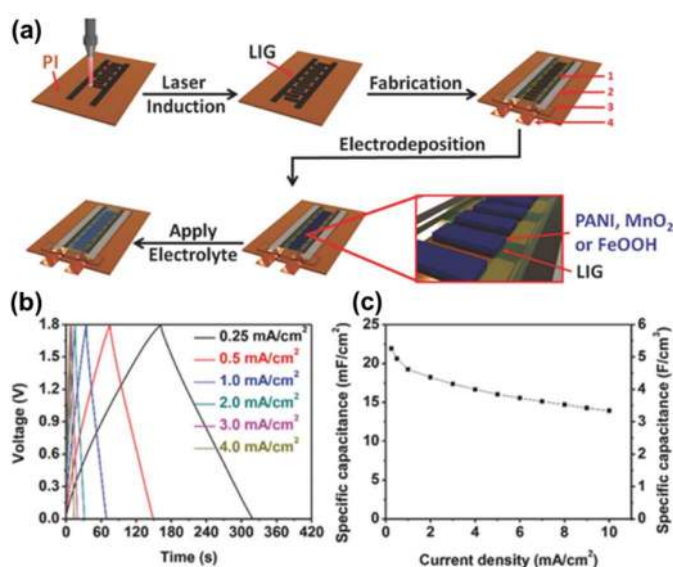
Fig. 8 In-plane LIG-FeOOH//LIG-MnO 2 AMSCs. (a) Scheme of the fabrication of MSCs with LIG-MnO 2 , LIG-FeOOH, or LIG-PANI. (b) GCD curves of LIG-FeOOH//LIG-MnO 2 AMSCs at current densities ranging from 0.25 to 4.0 mA cm -2 . (c) Areal and volumetric capacitances of LIG-FeOOH//LIG-MnO 2 AMSCs at current densities of 0.25-10 mA cm -2 . Reproduced with permission. 209 Copyright 2016, John Wiley & Sons, Inc.
