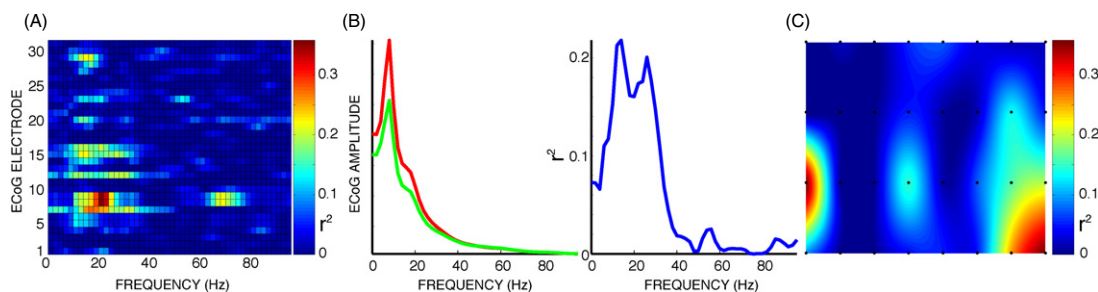
Figure 3. Example of an analysis comparing ECoG signals for the right-hand movement and rest (modified from [36]). (A) Color-coded values of r^2 for all locations and frequencies. (B) Average spectra (red for rest, green for the right-hand movement) (left) and r^2 as a function of frequency (right) for electrode 15. (C) Topographical distribution (black dots indicate electrode locations on the 8 \times 4 grid) for color coded r^2 values calculated for 20 Hz.
