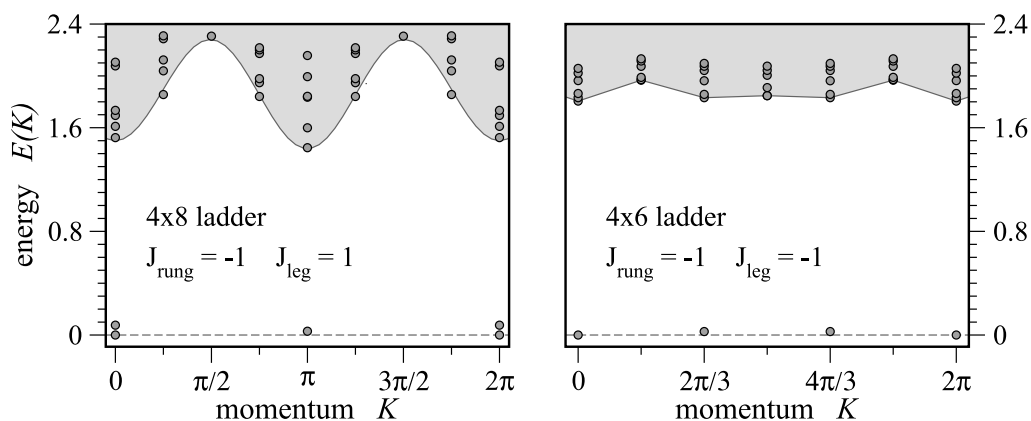
Figure 6. Gapped energy spectra of four-leg \text{su}(2)_3 anyonic ladders in a toroidal geometry versus the momentum along the legs.
