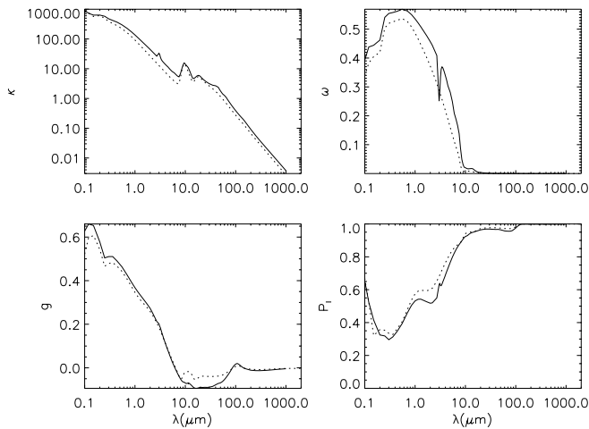
FIG. 1.—Behavior of the R_V = 4 grains with wavelength. For comparison, the dotted lines show behavior of ISM grains ( R_V = 3.1 ). Top left: Opacity, \kappa ; top right: albedo, \omega ; bottom left: average cosine of scattering angle, g ; bottom right: maximum polarization, p_l .
