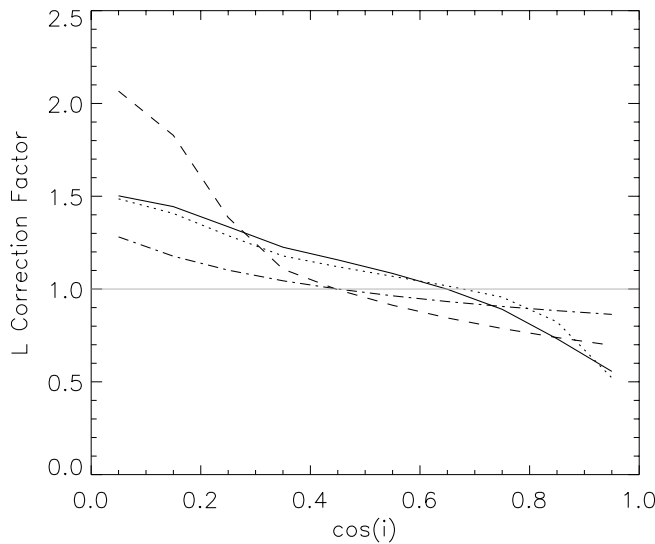
FIG. 10.—Luminosity correction factors as a function of inclination for the four geometries; model 1: dot-dashed line; model 2: dashed line; model 3: dotted line; model 4: solid line. These curves show the correction factor that would have to be applied to the integrated SED at a given inclination to correctly determine the source luminosity.
