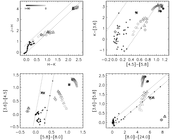
FIG. 12.—Color-color plots. The symbols correspond to the four models as follows. Model 1: filled circles; model 2: asterisks; model 3: open triangles; model 4: open diamonds. The models with cavities (3 and 4) are much bluer than the models without (1 and 2), despite their similar envelope masses (Table 2). The symbols are plotted at different levels of gray scale to indicate inclination, as shown by the gray-scale bar in the top left-hand panel. Edge-on sources are black, and pole-on sources are light gray. Notice that some of the bluest models are edge-on. This is due to the dominant contribution of scattered light to the source flux. These edge-on sources are very faint so would stand out in a color-magnitude diagram as faint and blue. The dotted lines are reddening vectors off the main-sequence and red giant branch (small crosses). The black dots along one of the reddening lines denote increments of A_V = 30 . The models in the bottom left-hand panel are well-separated from reddened main-sequence and giant stars. The models at bottom right are well-separated from stars with A_V less than 100.
