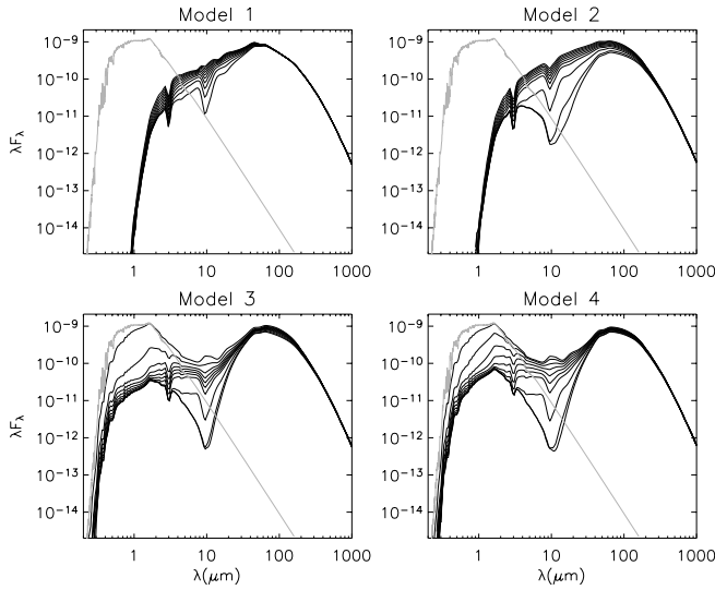
FIG. 9.—Spectral energy distributions for the four geometries. Fluxes (ergs cm -2 s -1 ) are scaled to a 1 L ⊙ source at a distance of 140 pc. Ten inclinations are plotted ranging from cos i = 0.05 to 0.95 at intervals of 0.1. The light gray line is the input stellar spectrum.
