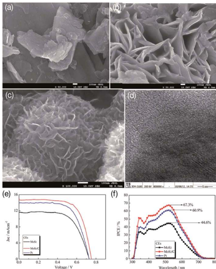
Fig. 10 Scanning electron microscopy (SEM) images of (a) commercial \text{MoS}_2 , (b) hydrothermal route synthesized \text{MoS}_2 , (c) porous \text{MoS}_2 -carbon hybrid prepared by a hydrothermal route, (d) high-resolution TEM image of \text{MoS}_2 -carbon hybrid, (e) photocurrent-voltage ( J - V ) curves of the DSSCs with \text{MoS}_2 , \text{MoS}_2 -C and Pt CEs and (f) incident photon-to-current efficiency (IPCE) spectra of the DSSCs with \text{MoS}_2 , \text{MoS}_2 -C and Pt CEs. Reprinted with permission from ref. 171, G. Yue, J. Wu, Y. Xiao, M. Huang, J. Lin and J. Y. Lin, high performance platinum-free counter electrode of molybdenum sulfide-carbon used in dye-sensitized solar cells. J. Mater. Chem. A , 2013, 1, 1495–1501. Copyright© Royal Society of Chemistry.
