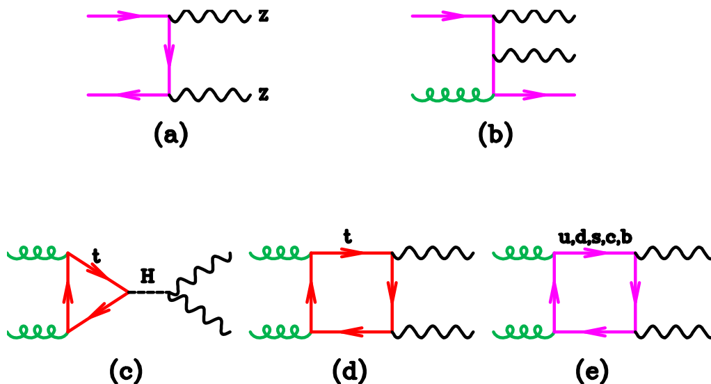
Figure 1. Representative diagrams for the ZZ production. In the following we will suppress the Z -decays to leptons.
