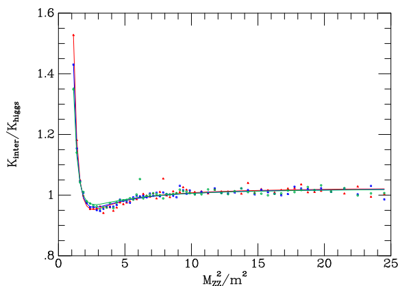
Figure 16. The ratio of the K -factors for the square of the Higgs diagrams alone ( K_{\text{higgs}} ) and the one for the interference ( K_{\text{inter}} ). The lines are fits to the individual histogram bins that are good to the level of a few percent and are shown for the central scale (blue) as well as the scale variations (red, green).
