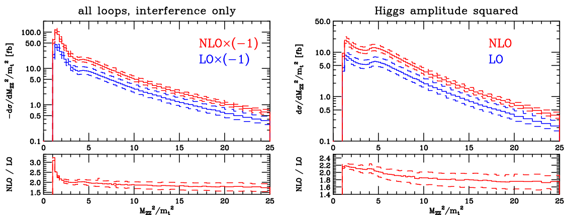
Figure 15. Left panel: interference of the Higgs amplitude and quark loops at LO and NLO, with the scale uncertainty indicated by the dashed histograms. The ratio of the NLO and LO results is shown in the lower panel. Right panel: the equivalent results for the Higgs amplitude squared.
