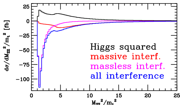
Figure 14. Comparison of the effect of the massless (magenta) and massive (red) loops in the NLO interference. Also shown is the sum (blue) and the corresponding result for the Higgs amplitude squared (black). All curves are computed for the central scale choice, \mu_r = \mu_f = M_{ZZ}/2 .
