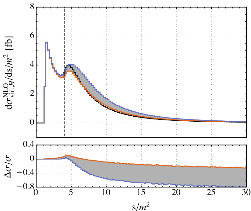
Figure 4. Virtual NLO corrections to gg \rightarrow H \rightarrow ZZ cross section with rescaling from eq. (2.26). See text for details. 1.) Exact NLO result (black). 2.) Varying orders of rescaled LMEs are indicated by shaded grey area. Its envelope is given by \sigma_{\text{imp,1}}^{\text{NLO}} (orange) and \sigma_{\text{imp,10}}^{\text{NLO}} (blue). The bottom plot shows the relative deviations with respect to the exact NLO results. The vertical dashed line denotes the top quark pair-production threshold.
