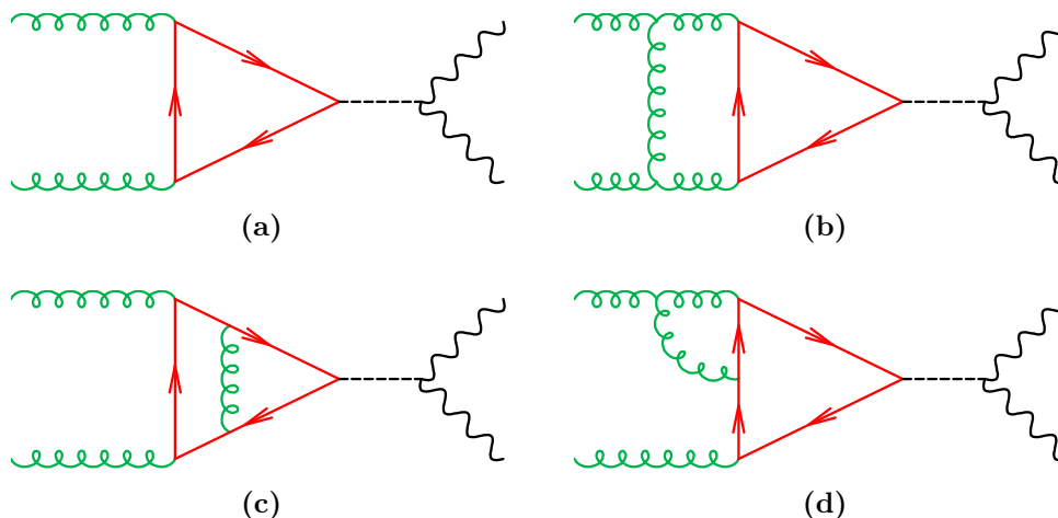
Figure 2. Representative diagrams for the LO+NLO virtual gg \rightarrow H \rightarrow ZZ amplitude.
