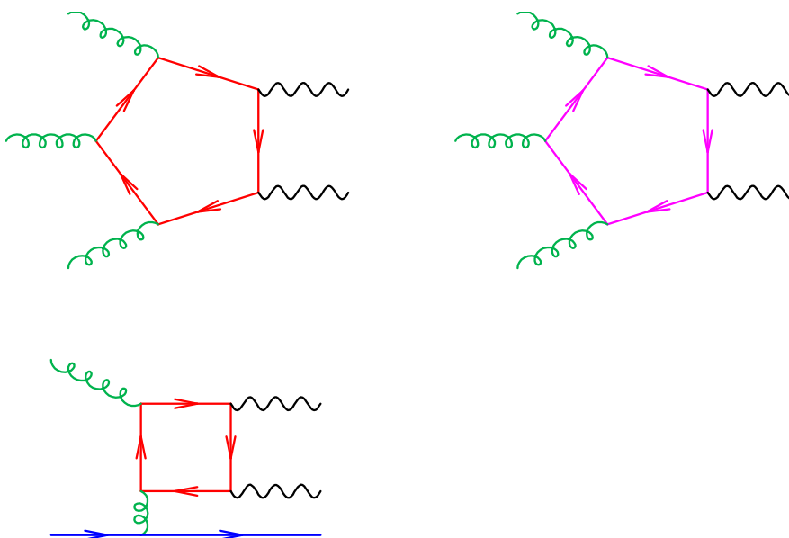
Figure 11. Representative diagrams for the 0 \rightarrow ggZZg and the 0 \rightarrow gZZq\bar{q} amplitudes.
