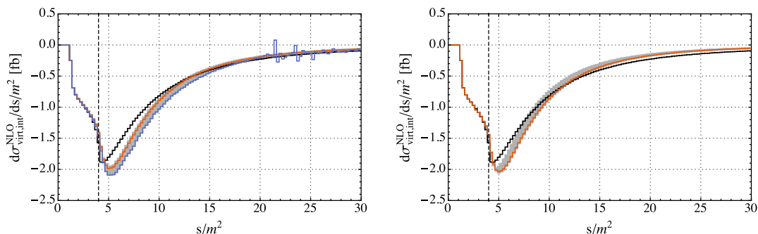
Figure 9. Next-to-leading-order interference \text{Re} \langle \mathcal{F}_A^{(1)}(m, \mu) | \mathcal{F}_B^{(2)}(m, \mu) \rangle . Left panel: interference by rescaling, eq. (2.26). Padé approximant [3/3] as comparison (black). Envelope of \sigma_{\text{imp},n}^{\text{NLO}} for n = \{1, \dots, 6\} as grey area; n = 1 (orange) and n = 6 (blue) shown explicitly. Right panel: interference by alternative rescaling, eq. (3.27). Padé approximant [3/3] as comparison (black). Grey area given by envelope of \sigma_{\text{imp},[n/m]}^{\text{NLO}} with n, m = \{2, 3\} ; [3/3] shown explicitly (orange). The vertical dashed line denotes the top quark pair-production threshold. See text for details.
