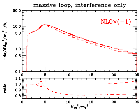
Figure 12. The uncertainty on the calculation of the massive loop interference contribution stemming from the use of the LME expansion and Padé approximants . The central result is shown as a solid histogram, with the dashed lines indicating deviations that correspond to the grey area in figure 9, multiplied by a factor of two. All curves are computed for the central scale choice, \mu_r = \mu_f = M_{ZZ}/2 .
