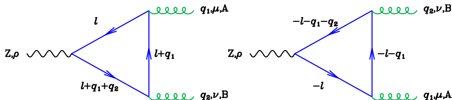
Figure 7. Triangle diagrams representing the Zgg form factor at lowest order.
