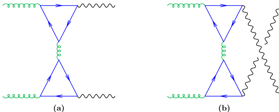
Figure 6. Two-loop anomaly style diagrams for the production of Z boson pairs.
