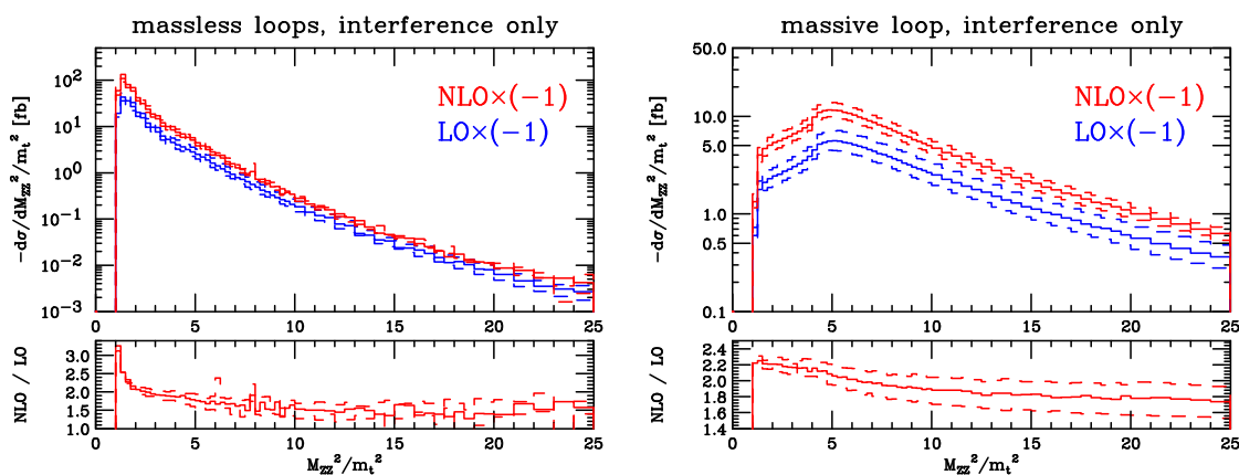
Figure 13. Left panel: interference of the Higgs amplitude and massless quark loops at LO and NLO, with the scale uncertainty indicated by the dashed histograms. The ratio of the NLO and LO results is shown in the lower panel. Right panel: the equivalent results for the interference of the Higgs amplitude and the top quark loops.
