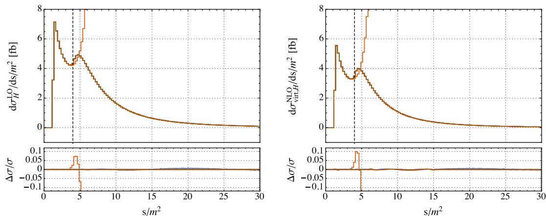
Figure 3. Left panel: leading-order gg \rightarrow H \rightarrow ZZ cross section. 1.) LME up to 1/m^{20} (orange). 2.) Exact result (black), LME with conformal mapping (blue) and Padé approximants [4/4] , [4/5] , [5/4] , [5/5] (yellow, purple, green, brown) agree perfectly. Right panel: virtual NLO corrections to gg \rightarrow H \rightarrow ZZ cross section. See text for details. Color code as in left panel. The bottom plots show the relative deviations with respect to the exact (N)LO results. The vertical dashed line denotes the top quark pair-production threshold.
