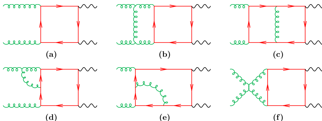
Figure 5. Representative diagrams for the LO and virtual NLO gg \rightarrow ZZ amplitude.
