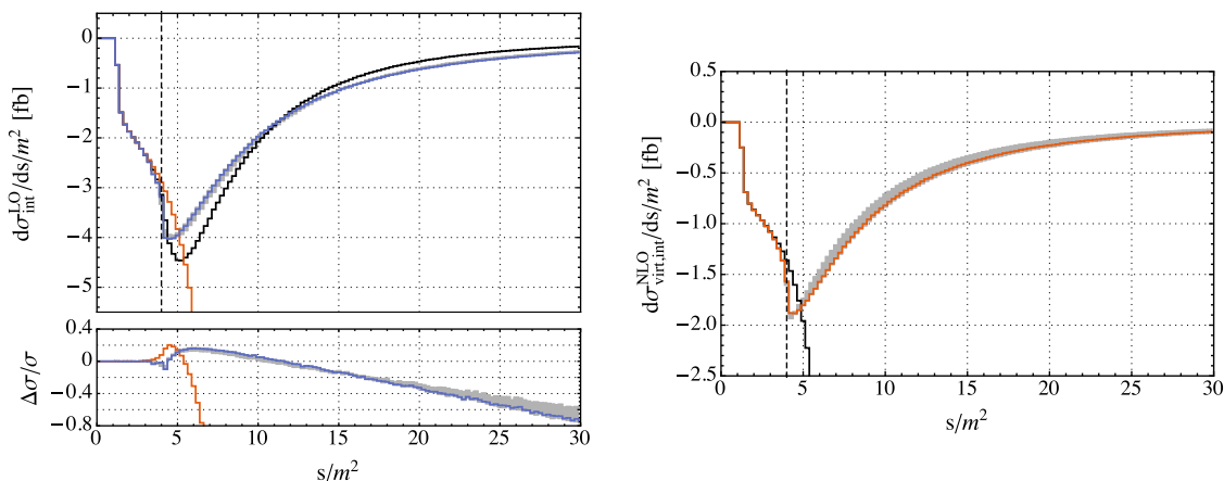
Figure 8. Left panel: leading-order interference \text{Re} \langle \mathcal{F}_A^{(1)}(m, \mu) | \mathcal{F}_B^{(1)}(m, \mu) \rangle . Exact result (black), LME up to 1/m^{12} (orange) and envelope of Padé approximants [2/2] , [2/3] , [3/2] and [3/3] (blue) as grey area. Bottom plot shows the relative deviation from the exact result. Right panel: next-to-leading-order interference \text{Re} \langle \mathcal{F}_A^{(1)}(m, \mu) | \mathcal{F}_B^{(2)}(m, \mu) \rangle . LME up to 1/m^{12} (black) and envelope of Padé approximants [2/2] , [2/3] , [3/2] and [3/3] (orange) as grey area. The vertical dashed line denotes the top quark pair-production threshold. See text for details.
