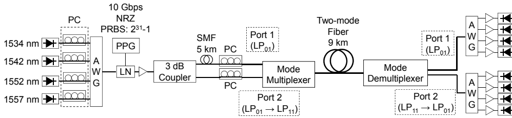
Fig. 10. Experimental setup for MDM-WDM transmission.
