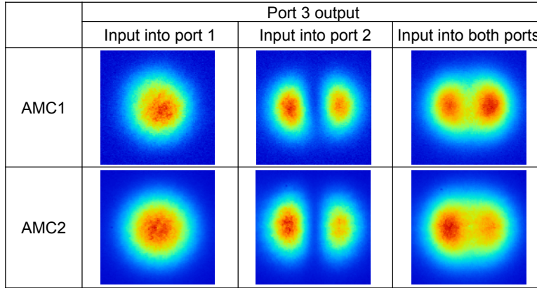
Fig. 7. Near field patterns of AMC1 and AMC2.
