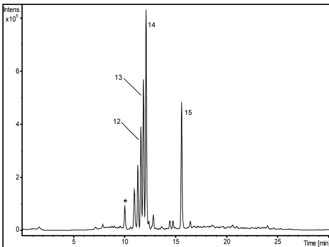
Fig. 4 Presence of bufadienolides in the \text{CH}_2\text{Cl}_2 soluble fraction of B. pinnatum : HPLC-APCIMS base peak chromatogram (positive ion mode, m/z 150 - 1500). SunFire TM \text{C}_{18} column, A: 0.1% aqueous formic acid and B: MeCN, 5-100% B in A in 30 min, 0.5 mL/min. Numbers refer to bufadienolides 12-15 . * This peak ( m/z 475.3) was tentatively assigned to bryophyllin C [34]. Peaks at R_t 11.0 min ( m/z 197.2) and R_t 11.3 min ( m/z 477.3, 459.3) were not identified.
