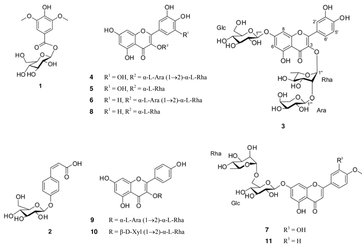
Fig. 2 Structures of compounds isolated from B. pinnatum
