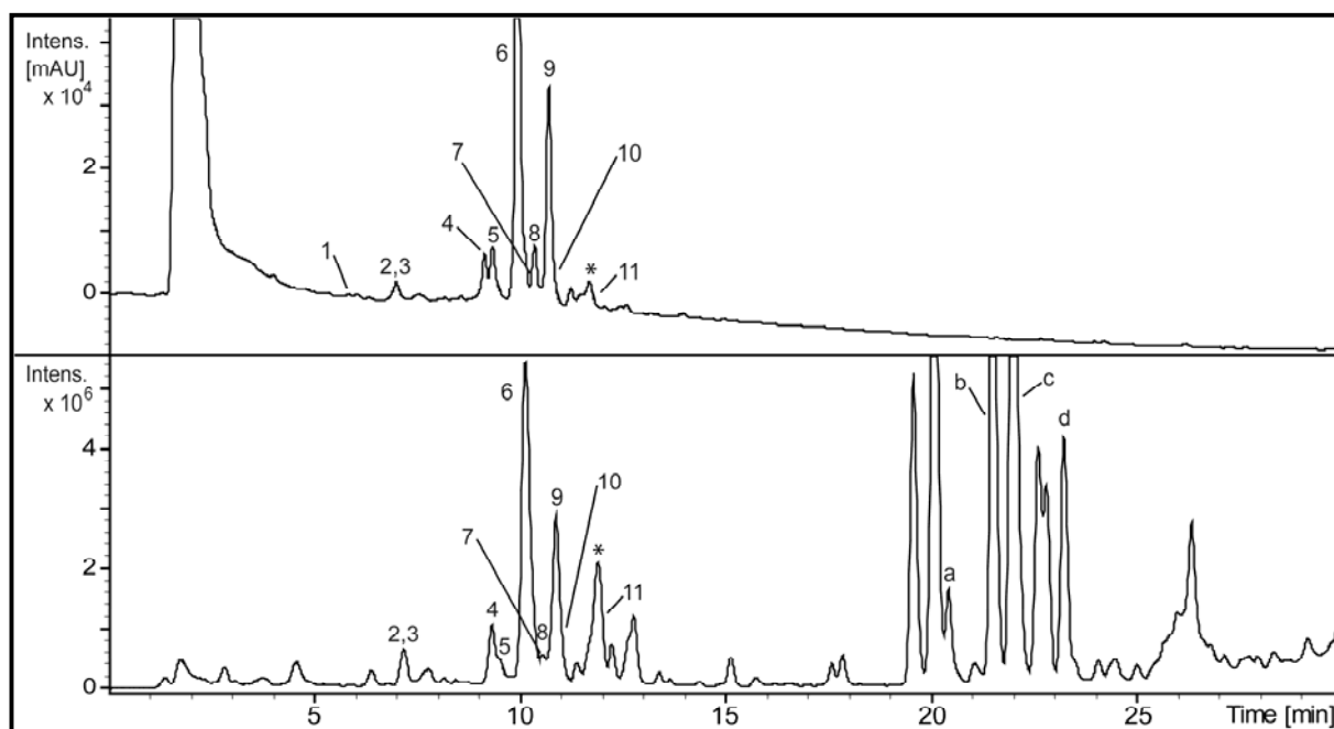
Fig. 1 HPLC-PDA-ESIMS of the MeOH extract of B. pinnatum . Top: UV trace (220-400 nm). Bottom: ESIMS base peak chromatogram (positive ion mode, m/z 200 - 1500). SunFire™ C 18 column, A: 0.1% aqueous formic acid and B: MeCN, 5-100% B in A in 30 min, 0.5 mL/min.
