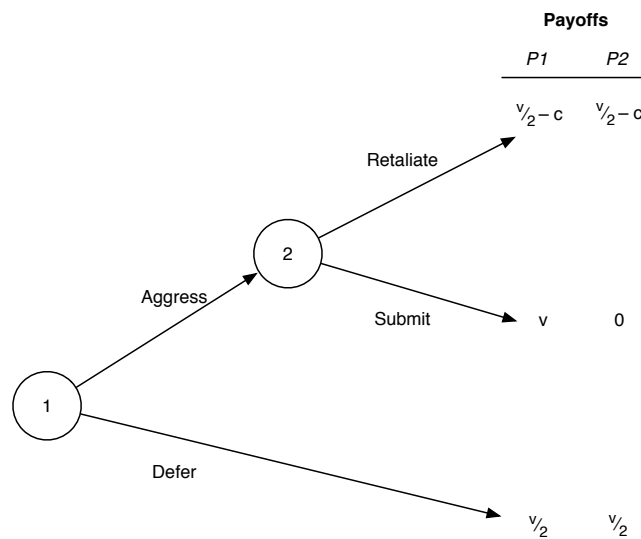
Figure 2. Sequential hawk-dove game. Assuming 2c > v , the only equilibrium is (Aggress, Submit).
