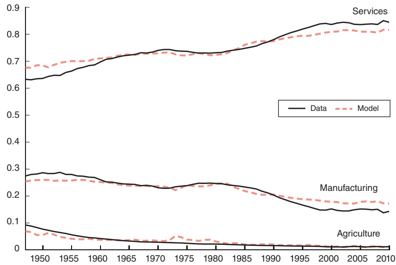
FIGURE 13. FIT OF HOMOETHETIC SPECIFICATION IN COLUMN 3
