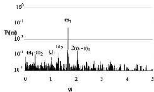
FIG. 9. Spectrum obtained at Re/Re_{c1}=7.2 for cavitating condition at Pe=3000 Pa.
