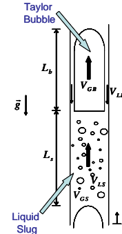
Figure 12. Geometry of a slug unit.
