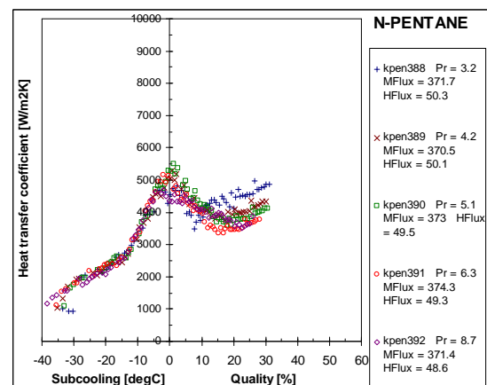
Figure 5. Heat transfer coefficient as a function of the equilibrium quality (saturated region) and of subcooling (subcooled region) in flow boiling of n-pentane (Kandlbinder, 1997).
