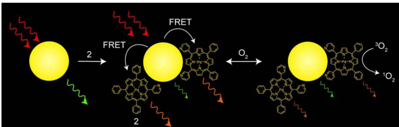
Figure 1. Schematic representation of the O 2 sensing transduction mechanism of a self-assembled Pd porphyrin ( 2 )-QD construct. The QD acts as the two-photon antenna of NIR (700–1000 nm) excitation. The QD emission is quenched in the presence of a surface-bound Pd porphyrin ( 2 ) via a FRET mechanism. The insensitivity of the QD emission to O 2 affords an internal reference to establish a ratiometric O 2 response.
