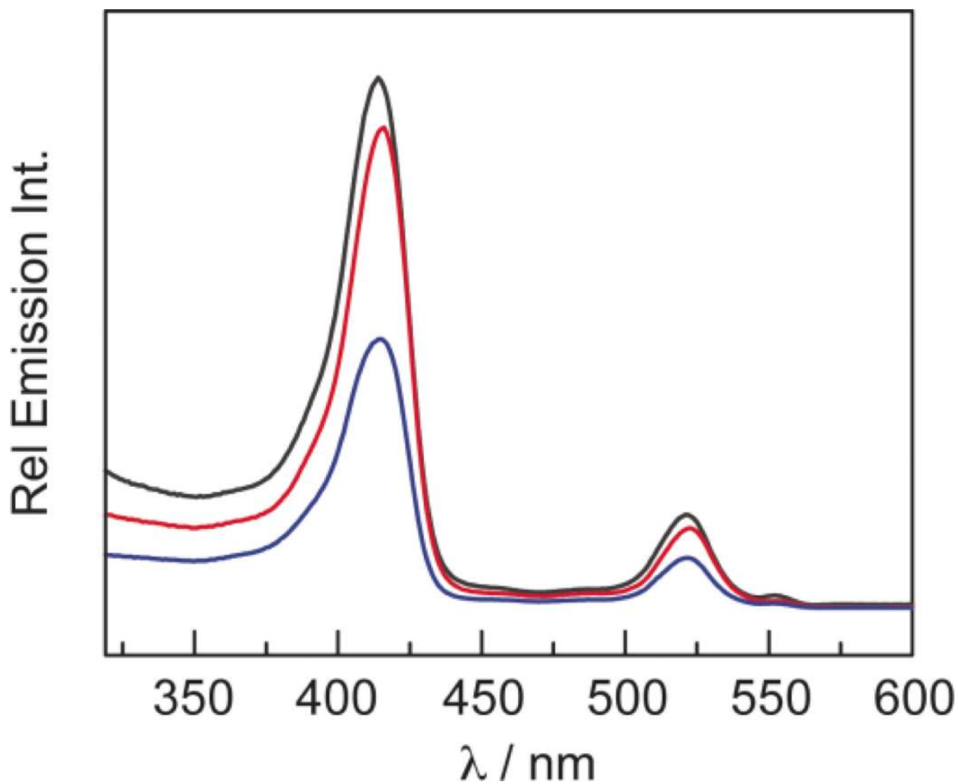
Figure 8. Excitation spectra ( \lambda_{\text{em}} = 685 \text{ nm} ) of concentration-matched toluene solutions of QD1 (—), QD2 (—) and QD3 (—).
